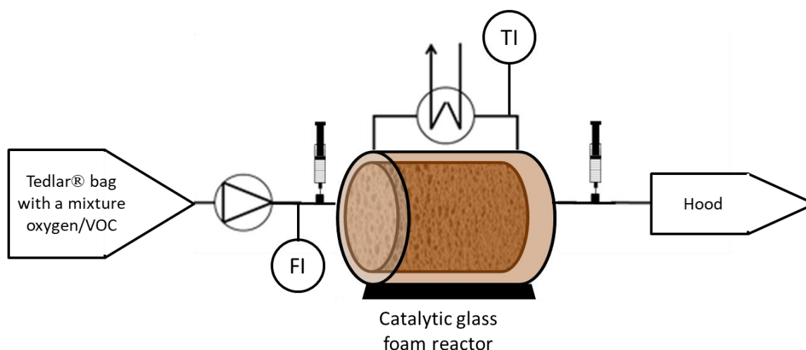
Figure 1. Layout of the setup for thermocatalytic oxidation of VOCs with a catalytic glass foam – TI: Temperature Indicator – FI: Flowrate indicator
