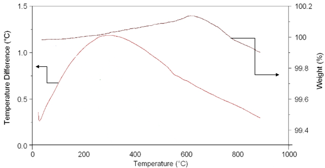
Figure 3. DTA-TGA curves obtained for the catalytic glass foam under air
