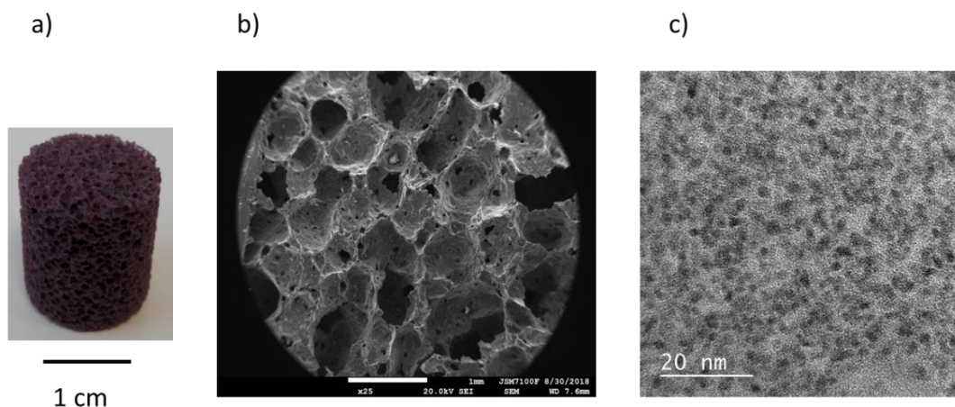
Figure 2. Real photo (a), SEM picture (b) and TEM picture (c) of the catalytic glass foam impregnated with ruthenium nanoparticles
