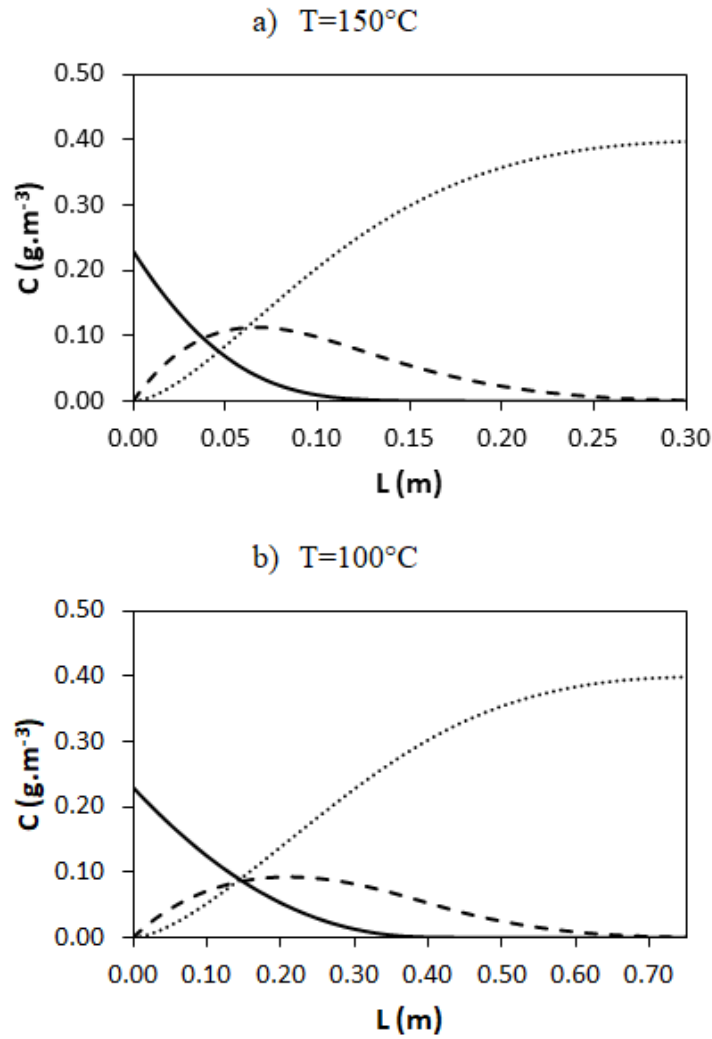
Figure 35. Concentrations of ethanol (full line), acetaldehyde (dashed line) and \text{CO}_2 (pointed line) along the reactor simulated for v=0.010 \text{ m}\cdot\text{s}^{-1} and ethanol inlet concentration of 140 ppmv ( 0.23 \text{ g}\cdot\text{m}^{-3} ) – a) T=150^\circ\text{C} – b) T=100^\circ\text{C}
