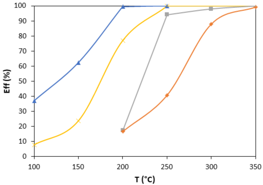
Figure 24. Removal efficiency of VOCs versus temperature ( v = 10 \text{ mm.s}^{-1} – residence time = 8.8 s) - ▲ : ethanol (inlet concentration: 1.0 \text{ g.m}^{-3} ) - × : acetone (inlet concentration: 2.0 \text{ g.m}^{-3} ) - ■ : toluene (inlet concentration: 1.0 \text{ g.m}^{-3} ) - ◆ : heptane (inlet concentration: 1.0 \text{ g.m}^{-3} )
