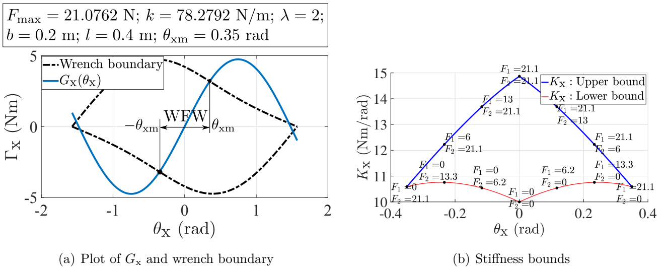
Figure 7: Wrench-feasible workspace (left) and stiffness bounds (right) for the X-joint.
