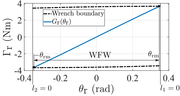
(a) Plot of G_r and wrench boundary
