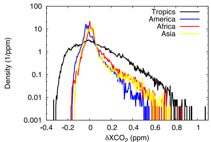
Fig. 1. Density function, in log scale, of the X_{\text{CO}_2} perturbations induced by perturbations of the carbon budget of 2.5, 0.9, 0.9, and 0.9 Gt C evenly spread over the tropical continents, over tropical America, over tropical Africa, and over tropical Asia, respectively. Each source is compensated with a sink of the same amplitude outside the tropical continents or in the same latitude band, including the oceans. X_{\text{CO}_2} values are simulated at the location of the OCO-2 retrieval used by Liu et al. The vertical weighting specific to each retrieval has been applied.
