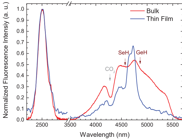
Fig. 2. IR fluorescence spectrum of Ga-Ge-Sb-Se thin film doped with 10000 ppmw of \text{Pr}^{3+} compared to that of corresponding bulk glass with excitation at 1.55 \mu\text{m} .
