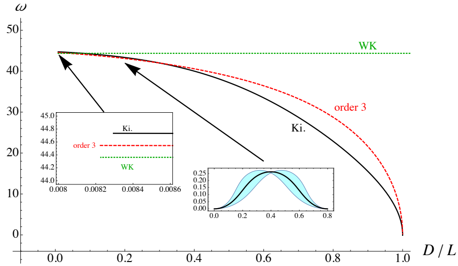
Figure 5: Vibration curve showing the frequency \omega vs axial displacement d for the second vibration mode, for \eta = 1/4800 . The curves for the Kirchhoff model (noted Ki.), the Woinowsky-Krieger model (noted WK), the order 3 model of Section 5 (noted order 3) are shown. (Inset) The equilibrium shape is plotted with the second vibration mode, for d = 0.2 . Note that \Omega = \omega / (L^2 \sqrt{\rho A / (EI)}) is the physical angular frequency in radians per second.
