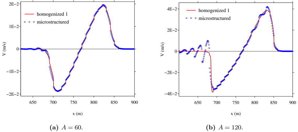
Figure 10: Superposition of the fields V_h and V^{(1)} at t = 0.16 s with close-up on the right-going waves in the case of a homogeneous periodic cell and a source at central frequency f_c = 10 Hz (i.e. \eta = 0.26 ), for two different amplitudes.
