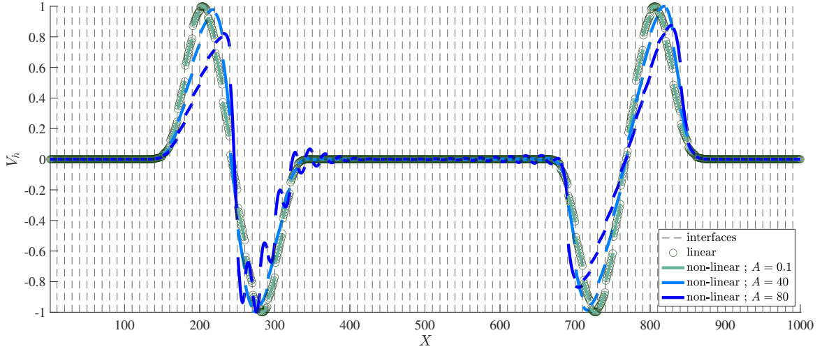
Figure 2: Snapshots of the wavefields V_h normalized at t = 0.16 s, which are simulated within a microstructured medium with a homogeneous periodic cell and containing either linear or non-linear interfaces (represented by vertical dashed lines). The corresponding physical parameters are provided in Section 5.3. The medium is excited by a source of central frequency f_c = 10 Hz and a varying amplitude A .
