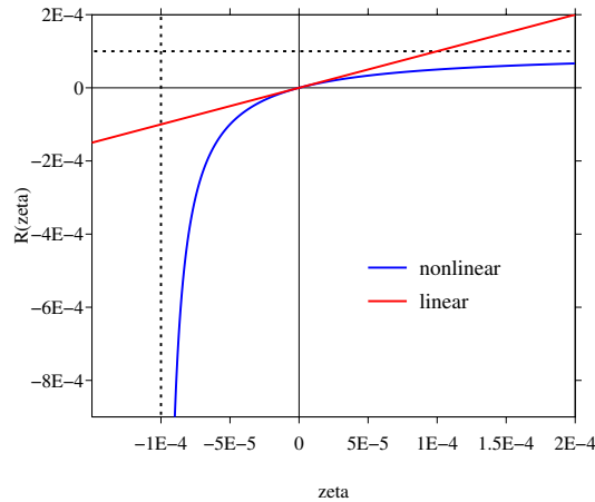
Figure 1: Hyperbolic interface law (5) and linear approximation. The dotted lines are placed at \zeta = -d and \mathcal{R} = d .
