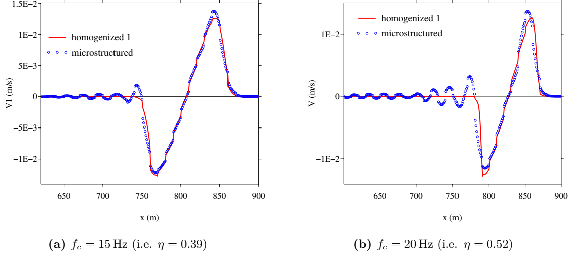
Figure 9: Superposition of the fields V_h and V^{(1)} at t = 0.16 s with close-up on the right-going waves in the case of a homogeneous periodic cell and a source of amplitude A = 40 , for two different central frequencies.
