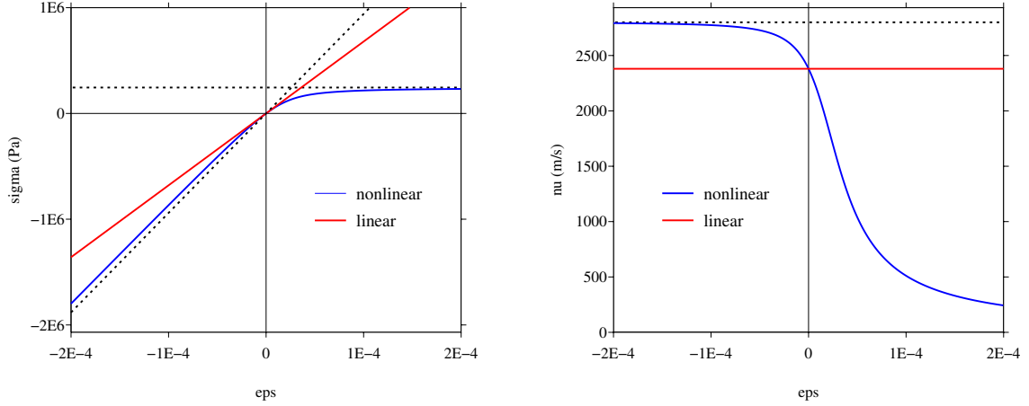
(a) Non-linear constitutive relation \Sigma_0 = \mathcal{G}_{\text{eff}}(\mathcal{E}_0) in (61) and linear case \Sigma_0 = \mathcal{C}_{\text{eff}}^\ell \mathcal{E}_0 in (32). (b) Sound speeds \nu_+(\mathcal{E}_0) in (64) and \nu_+^\ell for the linear case.
