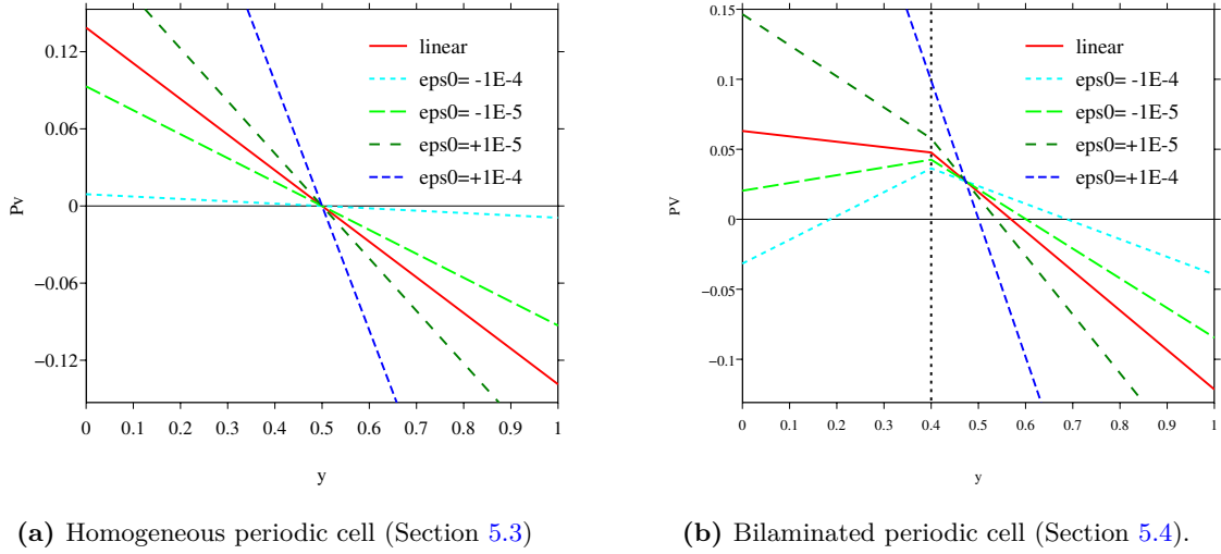
Figure 5: Velocity-based cell function \mathcal{P}_V(y, \mathcal{E}_0(X, t)) in (65) for various strain amplitudes \mathcal{E}_0 . The corresponding physical parameters are provided in the sections 5.3 and 5.4, respectively. In (b), the vertical dashed line indicates the position of the perfect interface between the two phases that constitute the bilaminated periodic cell.
