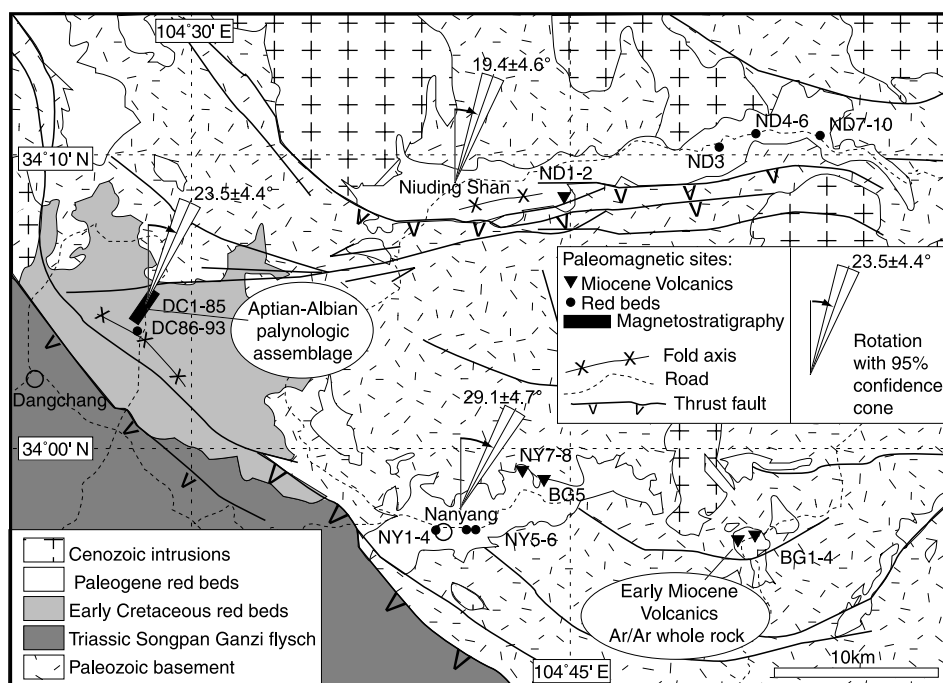
Figure 3. Simplified geologic map of the Dangchang area with sampling locations (with site identification numbers) and mean vertical axis rotations with respect to the APWP of Eurasia [Besse and Courtillot, 2002] for the Dangchang, the Nanyang, and the Niuding Shan localities.
