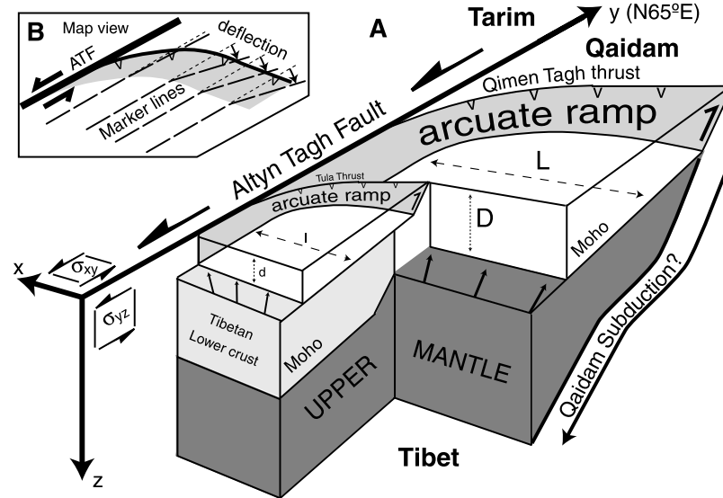
Figure 6. (a) Block diagram showing arcuate structures of different scales branching from the left-lateral Altyn Tagh fault (ATF). See Appendix A for definition of x , y , z , \sigma_{xy} , \sigma_{zy} , d , D , l and L . Expected compressional direction rotating with proximity to weak ATF are shown by arrows. (b) Map view showing predicted marker line deflection as thrust sheet passes over an oblique thrust ramp [Apostria et al., 1992; Wilkerson et al., 1992].
