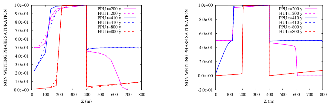
Figure 2: Non-wetting phase saturations as a function of z at different times t = 200, 410, 800 years, obtained for the TPFA PPU and HUI schemes on the 20 cells (left) and 200 cells (right) meshes.
