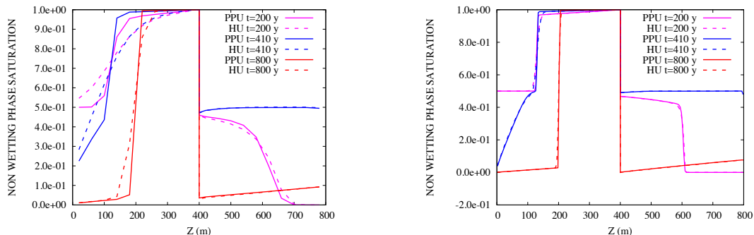
Figure 1: Non-wetting phase saturations as a function of z at different times t = 200, 410, 800 years, obtained for the TPFA PPU and HU schemes on the 20 cells (left) and 200 cells (right) meshes.
