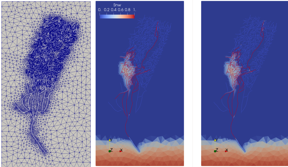
Figure 5: Left: triangular mesh of the DFM model with 32340 cells, 48558 faces and 5344 fracture faces (Courtesy of M. Karimi-Fard, Stanford, and A. Lapène, Total). Non-wetting phase saturation at final simulation time for the TPFA PPU (middle) and HUI (right) schemes.
