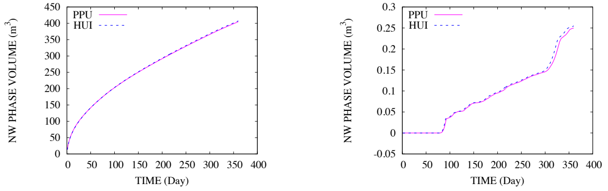
Figure 6: Volume of the non-wetting phase in the matrix (left) and in the fractures (right) as a function of time for the TPFA PPU and HUI schemes.
