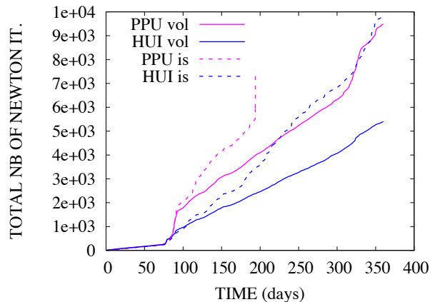
Figure 7: Accumulated number of Newton iterations as a function of time on (0, t_f) for the TPFA HUI and PPU schemes combined (is) or not (vol) with an interface nonlinear solver.
