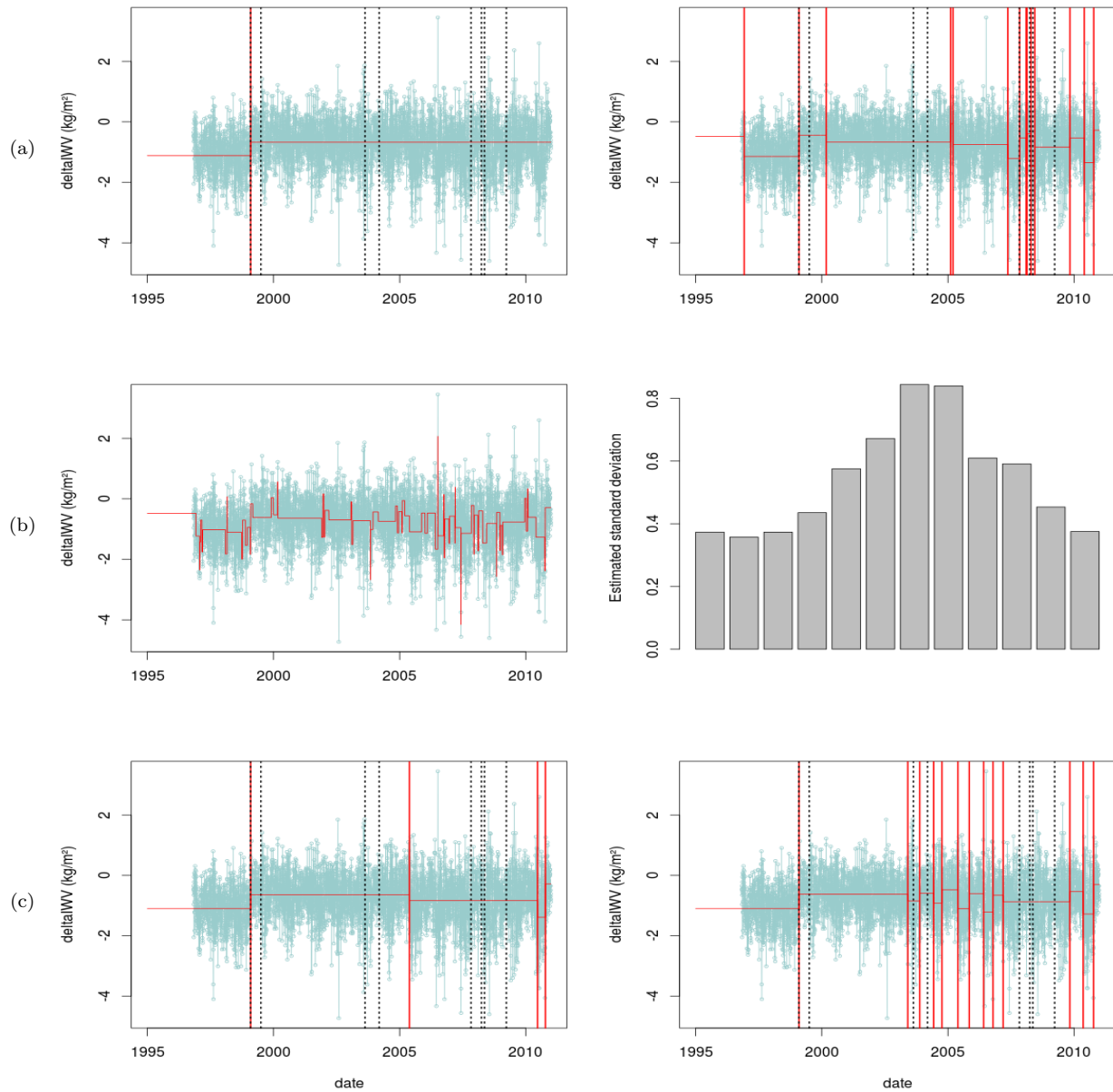
FIGURE 9. Results for the series ONSA. (a) the estimated breakpoints with \hat{K} = 2 (left: Lav and BM2) and \hat{K} = 15 (right: BM1). (b) the estimated mean with \hat{K} = 74 (left: mBIC) and the estimated standard deviation for each month (right). (c) the estimated breakpoints obtained with model MHomo (left: \hat{K} = 5 with Lav) and with model MHetero (left: \hat{K} = 14 with Lav). Solid lines (in red): the estimated breakpoints and the fitted expectation. Dashed lines (in black): known equipment changes (see Table 1).
