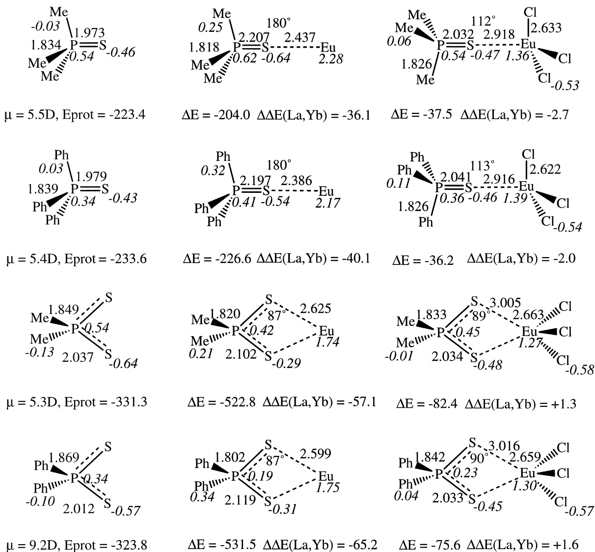
Fig. 2. See definitions in Fig. 1. L = \text{Me}_3\text{PS} ; \text{Ph}_3\text{PS} ; \text{Me}_2\text{PS}_2^- ; \text{Ph}_2\text{PS}_2^- .
