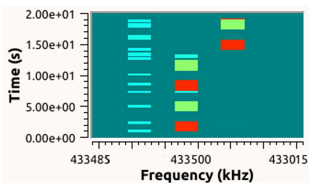
Fig. 3 Spectrum waterfall view on GRC received at gateway side in a 4 channels example (only 3 occupied in this picture), during experiments. Time is in y-axis (going down) and frequency in x-axis. Blue short transmissions are those produced by the traffic generator, green blocks are our IoT transmissions, and red blocks are the gateway transmissions itself
