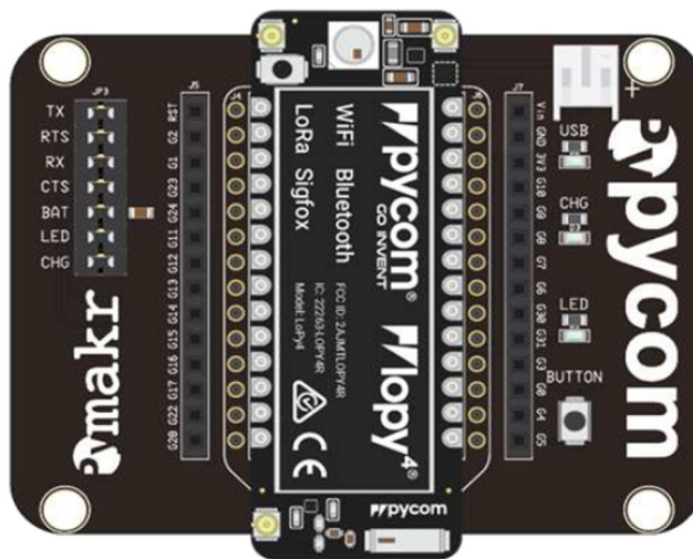
Fig. 7 Pycom module composed of a LoPy4 and an Expansion Board
