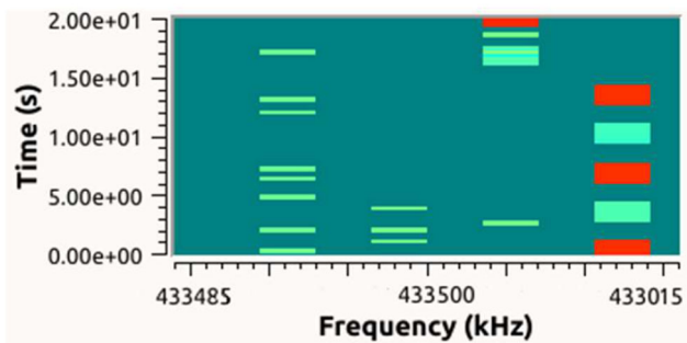
Fig. 4 Spectrum waterfall view on GRC received at IoTligent device side in a 4 channels example, during experiments. Time is in y-axis (going down) and frequency in x-axis. Green short transmissions are those produced by the traffic generator, red blocks are the IoT device transmissions, and blue blocks are gateway transmissions.
