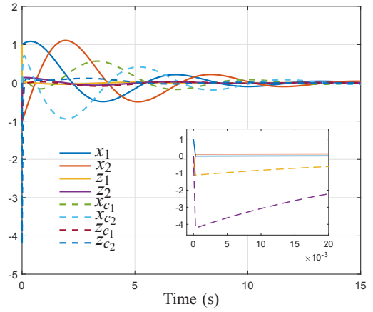
Fig. 1: State trajectories of the plant (solid line) and the controller (dashed line) with gains (38). The figure inset illustrates the trajectories of the fast variables z (solid line) and z_c (dashed line) in the initial period.
