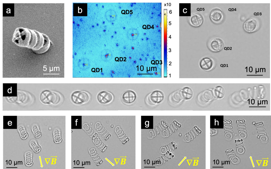
Figure 4. In-contact device and its controllable manipulation. (a) Scanning electron microscope (SEM) images of a micro-spring. (b) Fluorescent map of fabricated micro-spring structures with a integrated QD at the center of the micro-wheel before the development step. (c) The transmission optical microscope image of micro-spring structures corresponding to (b) the fluidic environment. (d) The transmission optical microscope images of a micro-spring at different bending stage when deliberately changing the direction of the magnetic flux in a semicircular track above the sample. (e–h) The orientation of structures toward higher gradient of magnetic field with depicted magnetic field gradient direction.
