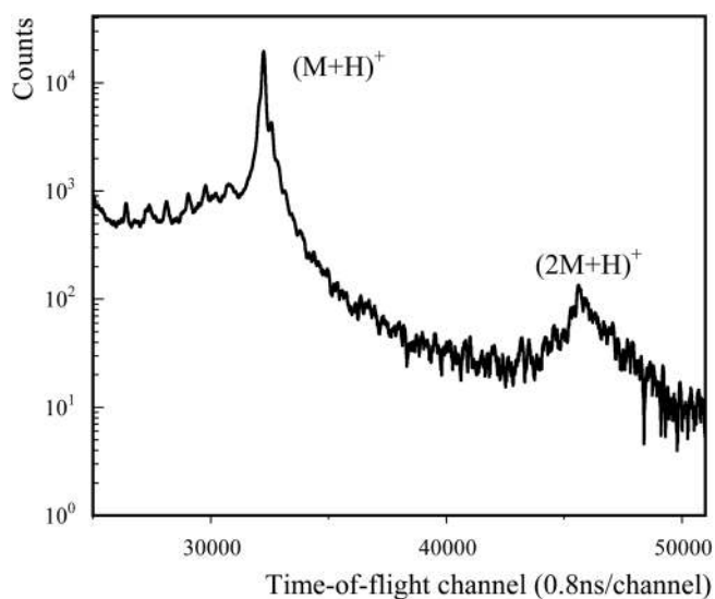
FIG. 8. Time-of-flight spectrum for a bradykinin deposit (dried sample from 2 \times 10^{-2} M solution in isopropanol) showing the presence of the bradykinin dimer ion. The spectrum is obtained with 3.67 \times 10^4 primary ions corresponding to a dose of 1.5 \times 10^7 nanoparticles/cm 2 .
