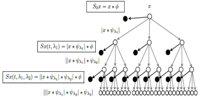
Fig. 2. Hierarchical representation of wavelet scattering coefficients at multiple layers [18].
