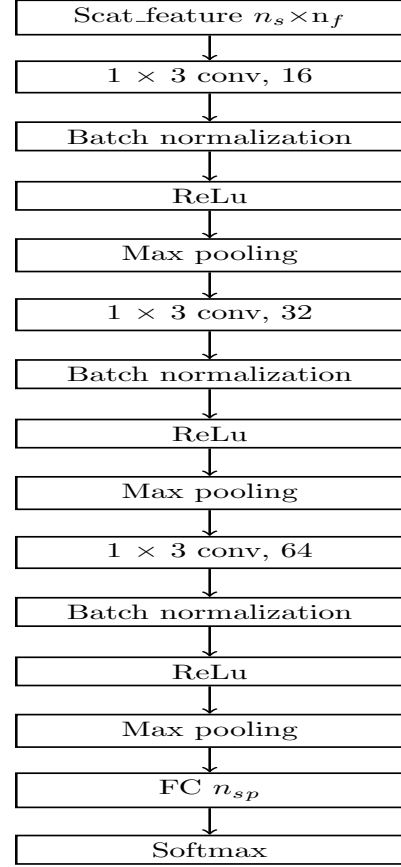
Fig. 3. Proposed Hybrid Network.
