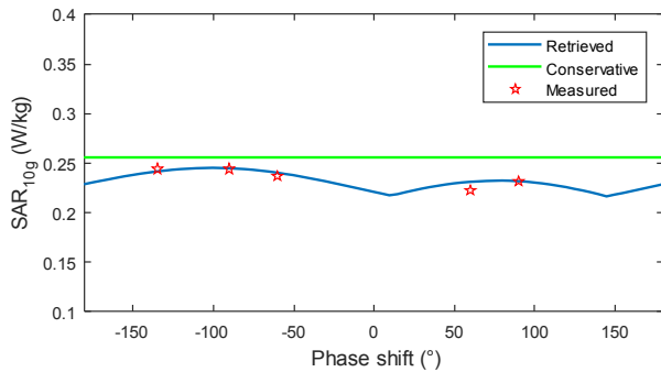
Fig. 11. Comparison between the retrieved (blue), the conservative (green) and the measured (red) SAR 10g values.
