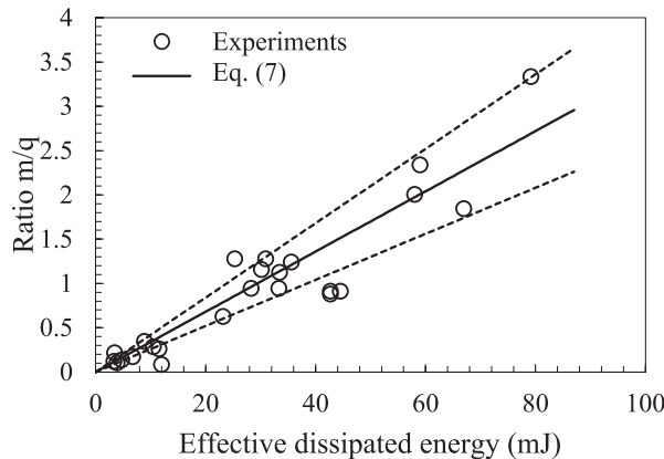
Fig. 17. Evolution of (a) the parameter n , (b) the ratio \frac{n}{m} , and (c) the ratio \frac{m}{q} as a function of the effective dissipated energy W (as-received material).
