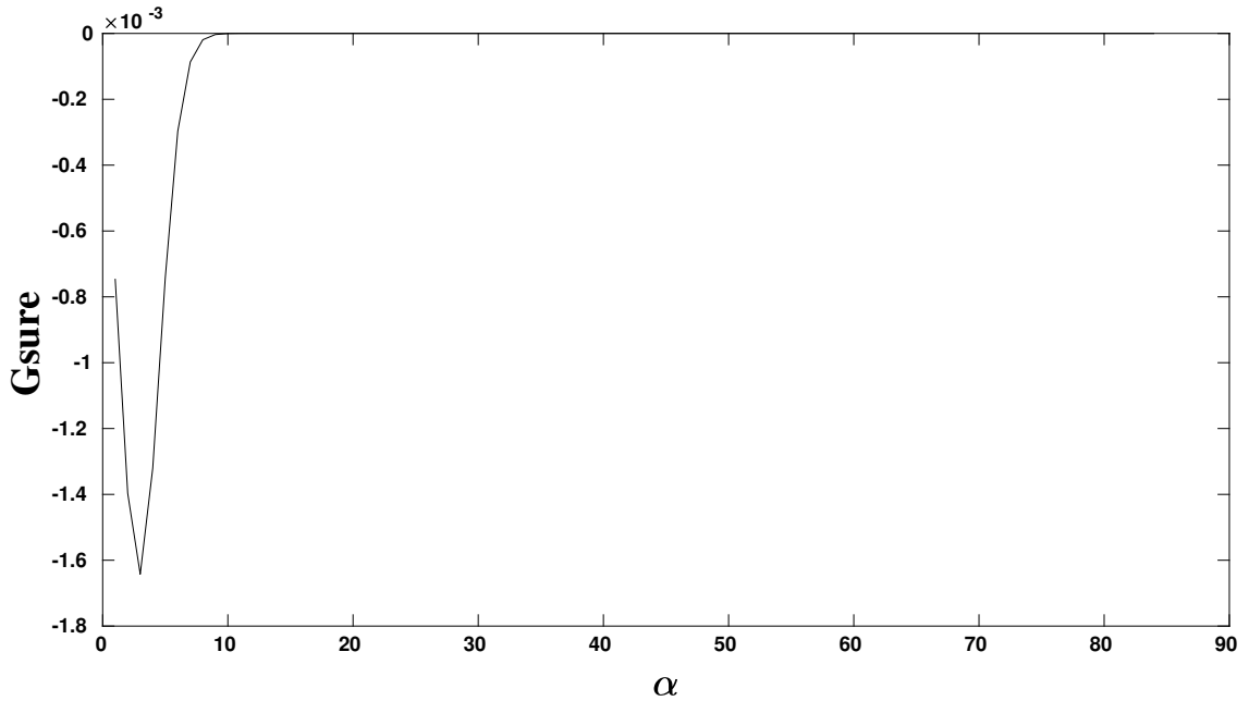
Figure 2: Typical evolution of the GSURE for the parameters n=128 , l=0.1 and \sigma = 0.1 .
