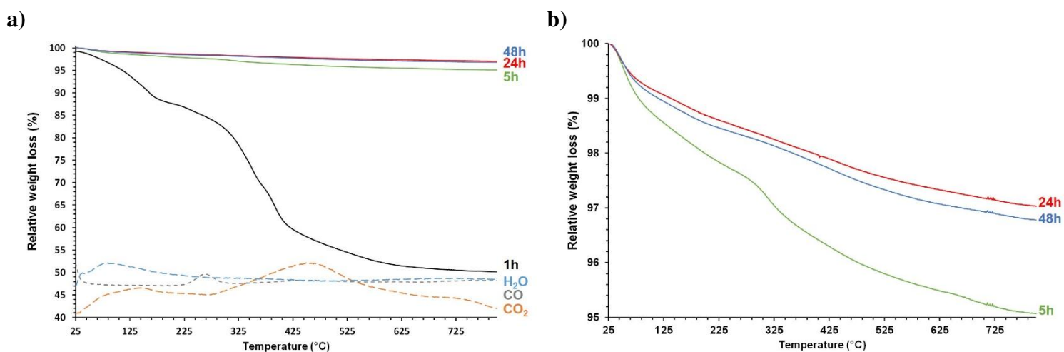
Figure 8. TG analyses of the samples formed through hydrothermal treatment of \text{Th}_2(\text{C}_2\text{O}_4)_5 \cdot n\text{H}_2\text{O} ( 250^\circ\text{C} , \text{pH} = 5 ) during 1h, 5h, 24h and 48h. Associated mass spectroscopy analysis of emitted gases is presented for the sample prepared after 1h ( \text{H}_2\text{O} : m/z = 18 - light blue dotted line; \text{CO}_2 : m/z = 44 - orange dotted line; \text{CO} : m/z = 28 - purple dotted line) (a). Focus of the curves obtained for 5h, 24h and 48h (b).
