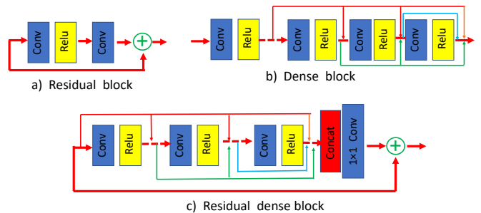
Figure 11: Comparison of different network blocks[42]. (a) Residual block in [43]. (b) Dense block in SRDenseNet [60]. (c) Residual dense block [42]
