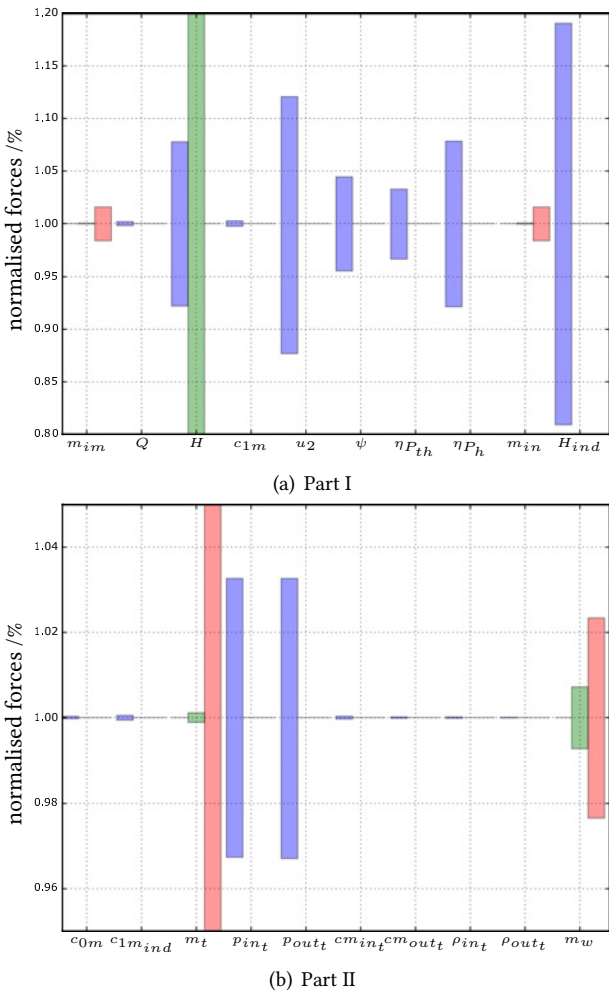
Figure 5. Results of normalised bearing loads on the fixed bearing for individual variation of input values, axial forces (blue), static radial forces (green), dynamic radial forces (red)
