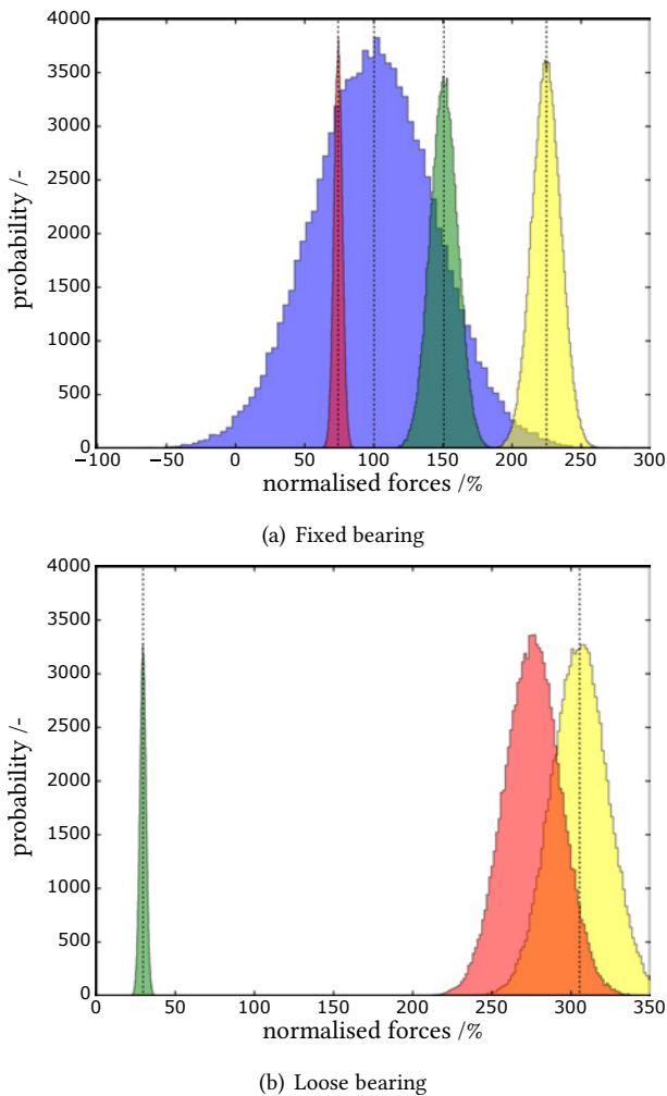
Figure 3. Results of bearing loads normalised by axial forces (blue), radial forces statically (green), dynamic radial forces (red), combined radial forces (yellow)
