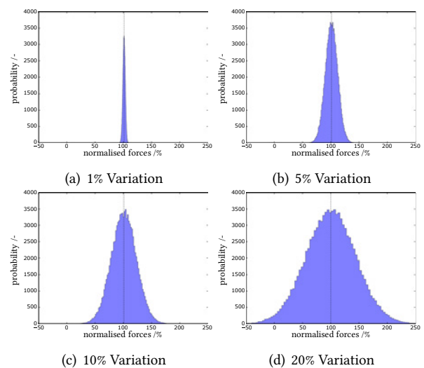
Figure 4. Influence of variation on axial forces
