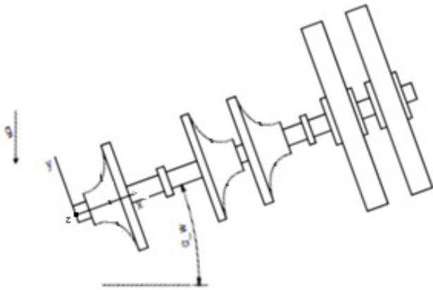
Figure 1. Example of turbopump configuration
