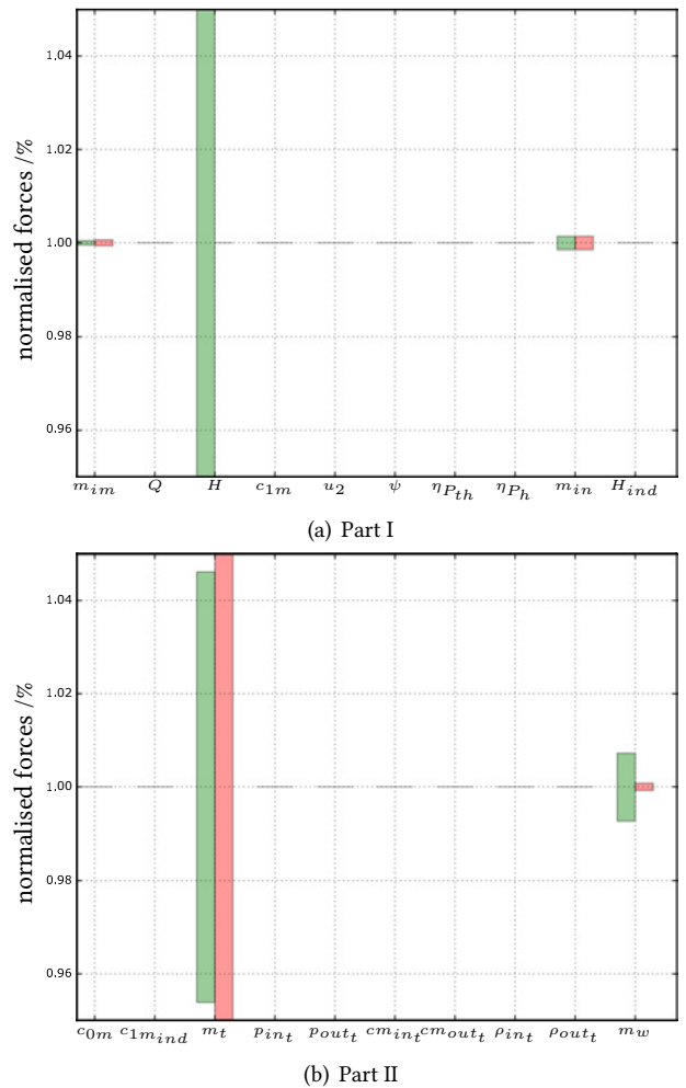
Figure 6. Results of normalised bearing loads on the loose bearing for individual variation of input values, radial forces statically (green), dynamic radial forces (red).
