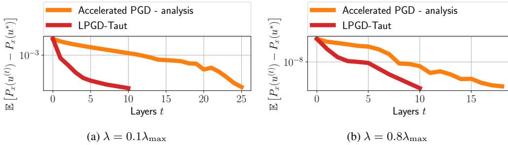
Figure 6: Performance comparison between LPGD-Taut and iterative PGD for the analysis formulation for the HRF deconvolution problem with fMRI data. Our proposed method outperform the FISTA algorithm in the analysis formulation. We notice a slight degradation of the acceleration in this high sparsity context.
