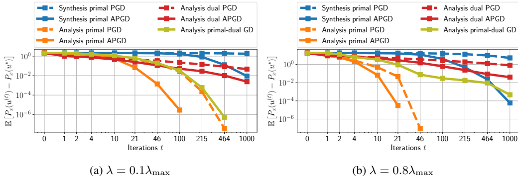
Figure 7: Performance comparison between the iterative solver for the synthesis and analysis formulation with the corresponding primal, dual or primal-dual re-parametrization. We notice that the primal analysis formulation provides the best performance in term of iterations. We also observe that the higher the regularization parameter, the faster the performance for each algorithm.
