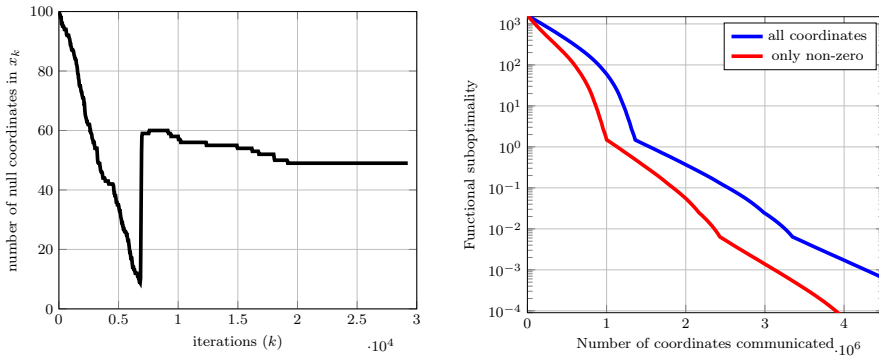
(a) Iterates density along a run of DAve-PG. (b) Suboptimality versus number of coordinates exchanged between machines.
