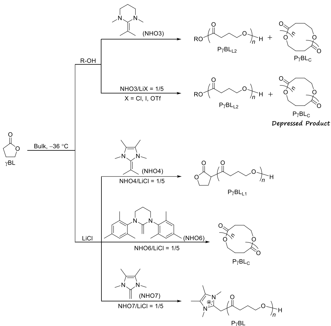
Scheme 12. ROP of \gamma BL by LiX/NHOs dual catalytic system [24].
