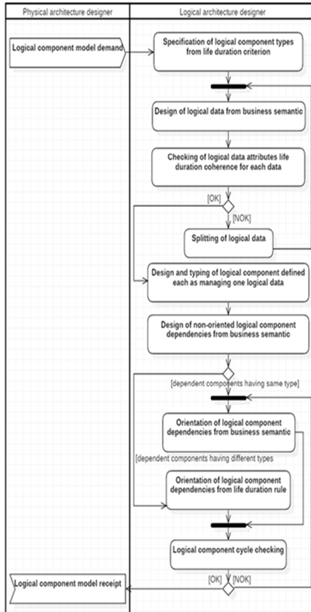
Fig. 7 - System-of-Services-Logical-Architecture-Design process.
