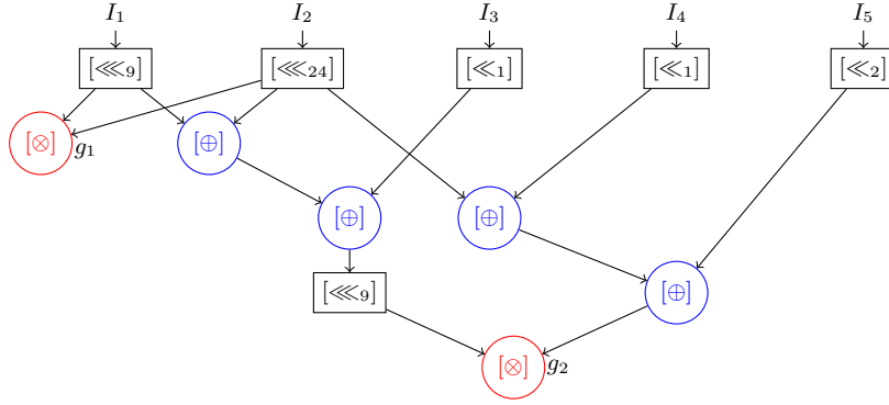
Fig. 6: Graph representation of a sub-circuit of Gimli.
