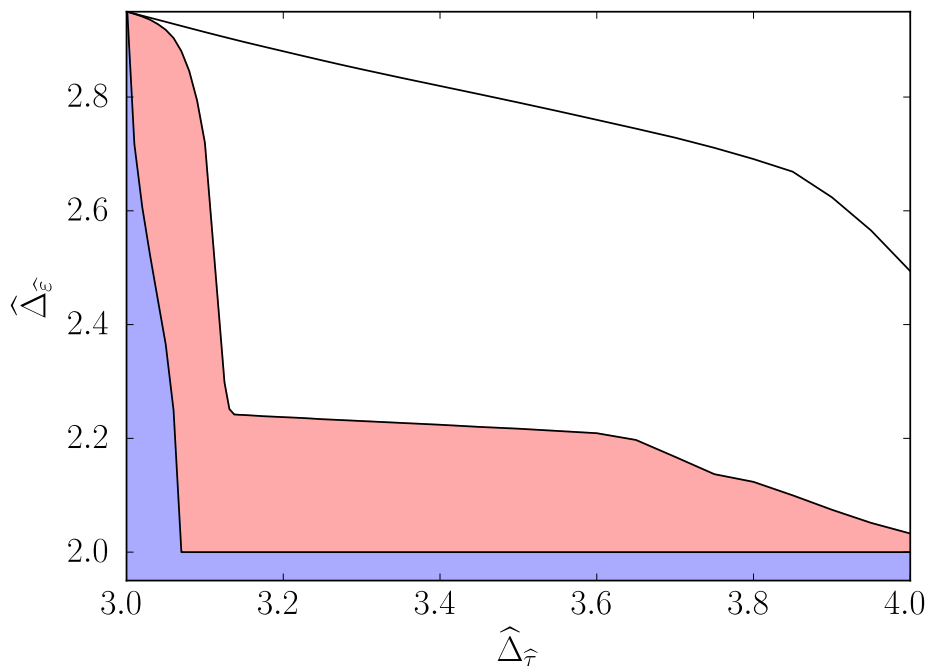
Figure 1. A plot showing the upper bound on the dimension of \hat{\epsilon} , the first scalar, other than the identity, seen by any of the OPEs in our correlator system. The unshaded region is the one that follows from a single correlator \langle \hat{O}_1 \hat{O}_1 \hat{O}_1 \hat{O}_1 \rangle . The pink region, which is more restrictive, uses the multi-correlator system but the only inputs it uses from the exact relations are the odd-spin operator dimensions given in table 1. The blue region, more restrictive again, follows from a genuine use of the exact relations. Since these depend on a_{\phi^2} , we have extremized \hat{\Delta}_{\hat{\epsilon}} over a third axis which is not shown.
