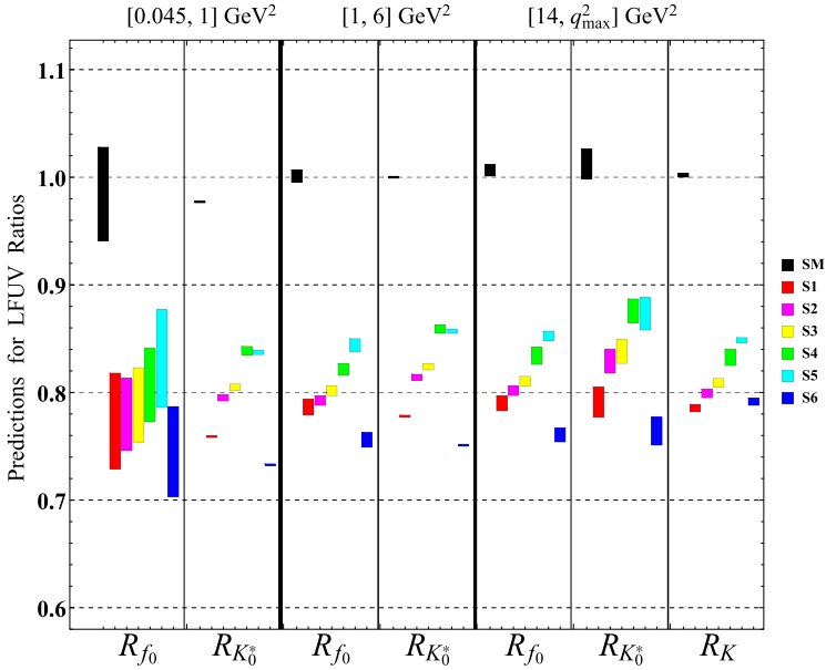
Fig. 1. Predictions for the LFUV ratios involving decays with scalar or pseudoscalar final state particles, R_{f_0} , R_{K_0^*} , and R_K . Three kinematical regions, low [0.045, 1] \text{ GeV}^2 , central [1, 6] \text{ GeV}^2 , and high [14, q_{\text{max}}^2] \text{ GeV}^2 , are chosen, where q_{\text{max}}^2 = 19.2, 14.9, and 22.9 \text{ GeV}^2 , for R_{f_0} , R_{K_0^*} , and R_K , respectively. In each case, predictions from left to right, correspond to the SM and scenarios S1 to S6, depicted with different colours.
