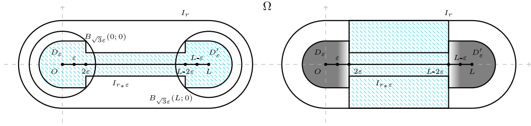
FIGURE 3. On the left the striped region corresponds to \text{supp}(\sigma_\varepsilon) , remark that the balls of radius \sqrt{3}\varepsilon centered respectively in (0; 0) and (L; 0) contain the modifications we have performed to satisfy the constraint. On the right we illustrate the level-lines of the cutoff function \tilde{z}_\varepsilon in grayscale.
