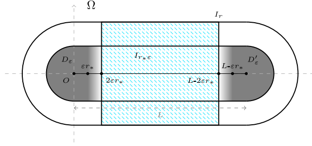
FIGURE 2. Illustration of the interval I and both its r and (r_*\epsilon) -enlargement for r_* \geq 1 . In grayscale we plot the levels of the function \zeta_\epsilon , whilst the striped region corresponds to the cylinder C_{r,\epsilon} .
