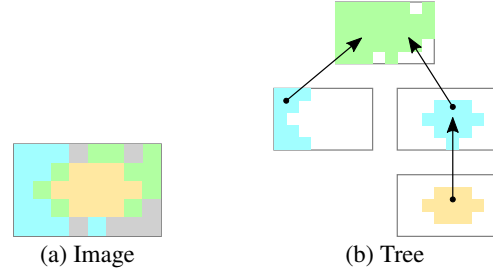
Figure 4. Perimeter data structure
