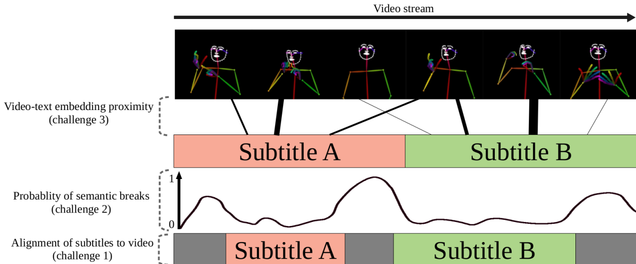
Figure 2: Illustration of challenges: alignment of text and video (challenge 1), semantic segmentation of sign language (challenge 2), and production of video-text embeddings for cross-modal retrieval (challenge 3)
