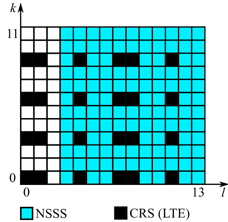
Fig. 9. Mapping of NSSS with one antenna port for NB-IoT, four antenna ports for LTE, and N_{ID}^{N_{cell}} = 0 for both systems.
