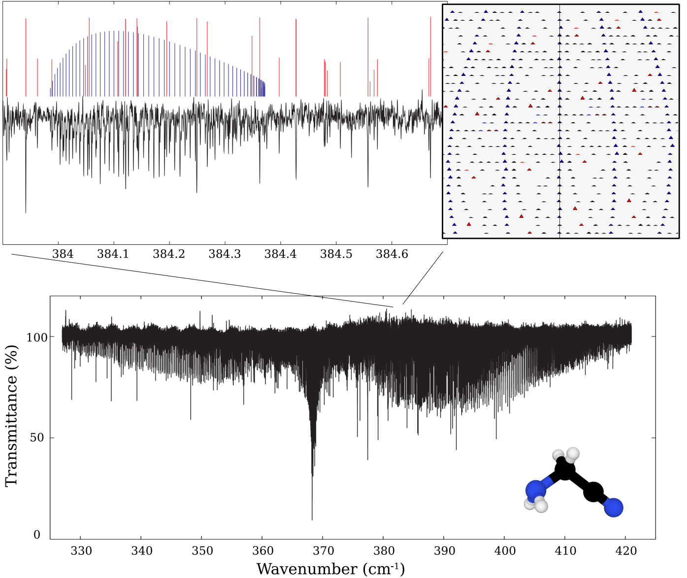
Fig. 1. Bottom panel: overview of the \nu_{17} band, centered around 368\text{ cm}^{-1} , recorded at 3\text{ }\mu\text{bar} pressure. Residual water lines were blanked out from the spectrum. The molecular geometry of aminoacetonitrile is also shown with carbon in black, nitrogen in blue, and hydrogen in white. Top left panel: detail of the {}^RQ_9 branch. The black curve is the experimental spectrum. The blue lines represent the position and the intensity of the {}^RQ_9 components, while the red lines represent other {}^RR transitions. Top right panel: Loomis-Wood diagram of the {}^RQ_9 branch using the same color legend. The wavenumber axis of the spectra ( x ) is plotted against consecutive J transitions across the y -axis; each row of the plot is 0.02\text{ cm}^{-1} wide. The height of the triangles is proportional to the spectral line intensity.
