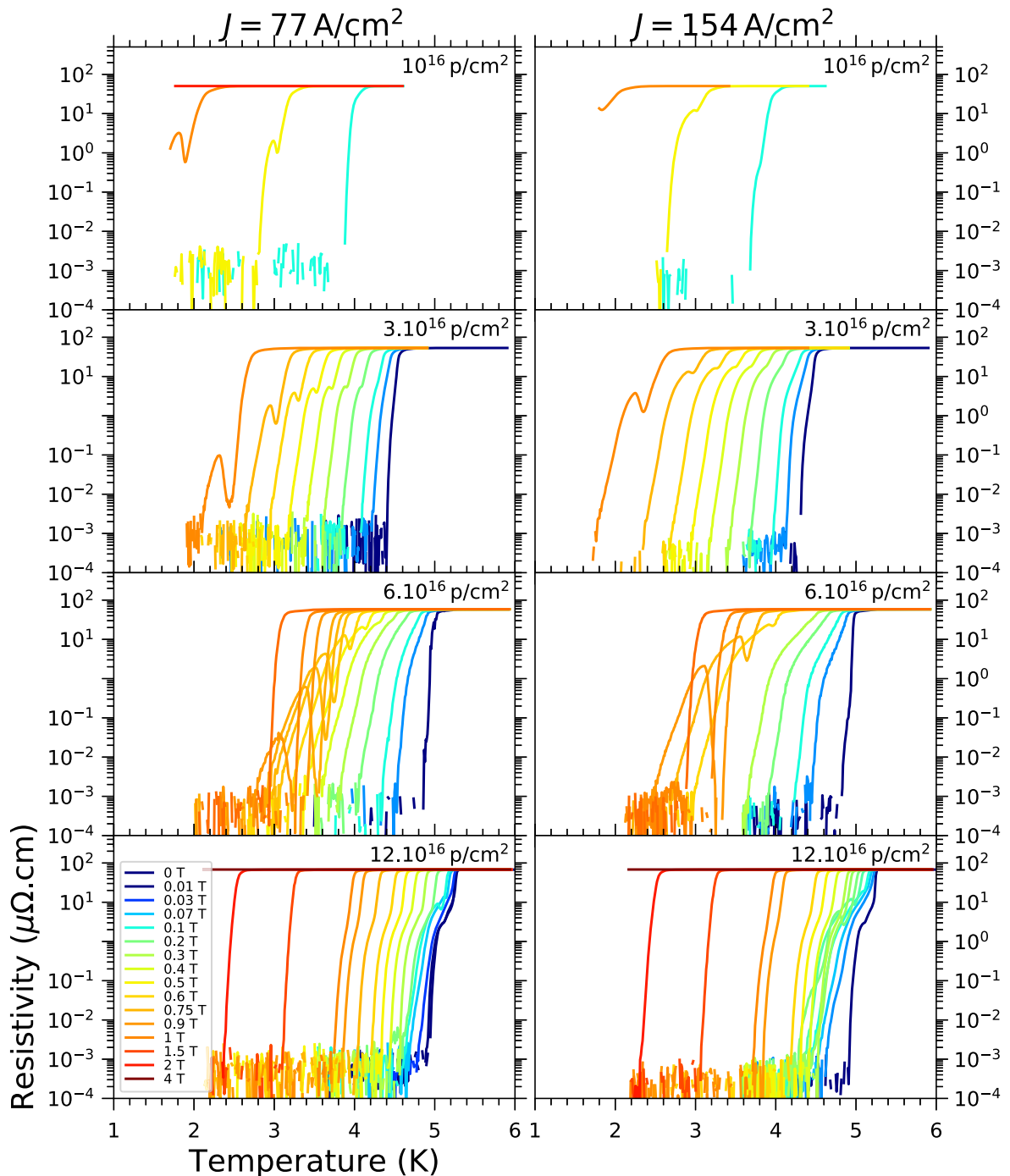
FIG. 7. Detailed magnetic field dependence ( H//ab ) of the c -axis resistivity of \text{Lu}_5\text{Ir}_4\text{Si}_{10} at the superconducting transition: for increasing irradiation doses (top to bottom) and using a current density of 77 (left column) and 154 \text{A}/\text{cm}^2 (right column). A peak effect is visible in the superconducting transition.
