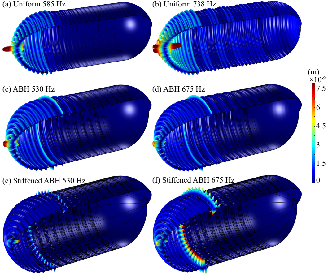
Figure 17: Displacement vibration shapes for (a)-(b) the uniform shells at the third stopband and fourth passband central frequency, (c)-(d) ABH shells, (e)-(f) stiffened ABH shells. Subfigures (c) and (e) correspond to the fifth stopband of the bare ABH structure, while (d) and (f) to its sixth passband. The stopbands and passbands have been selected for better illustrative purposes.
