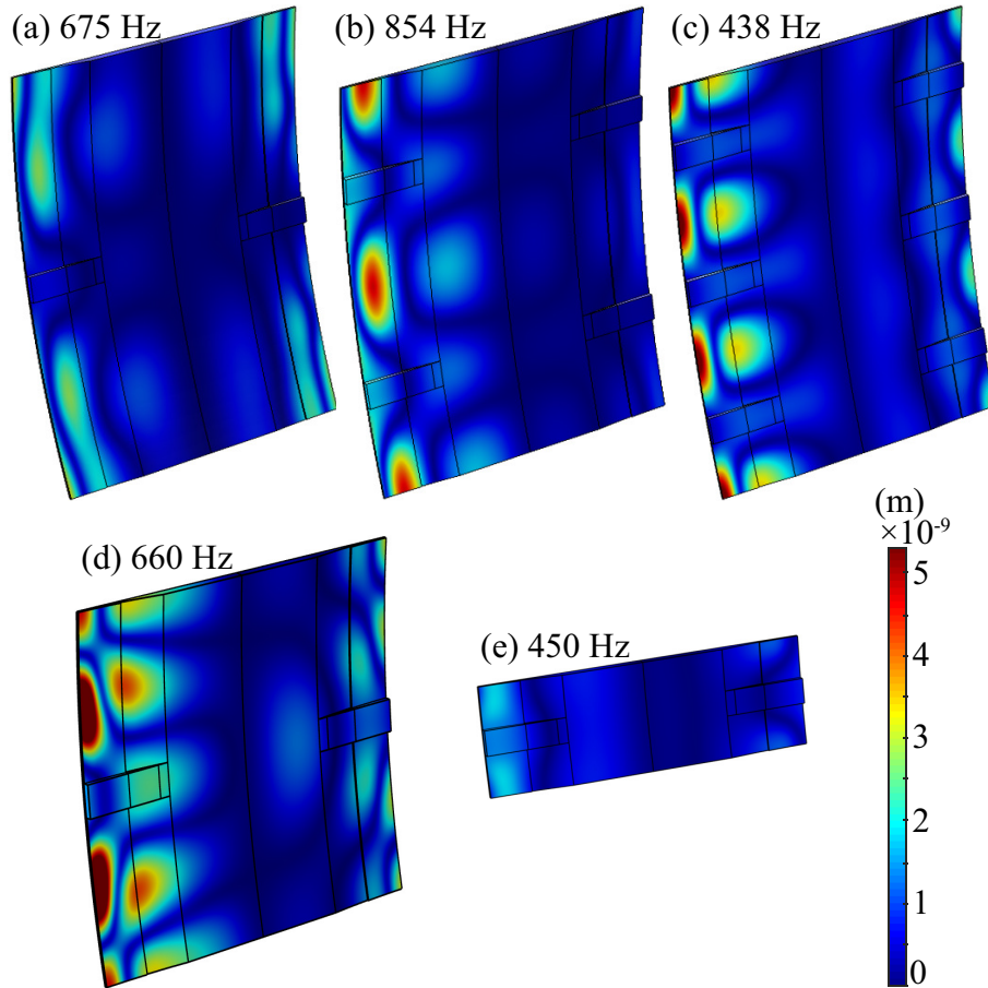
Figure 13: Displacement distribution for the rigid ABH shells with (a) 1 , (b) 2 and (c) 3 stiffeners for 1/16 section, (d) 1 stiffener for 1/24 section and (e) 1 stiffener for 1/60 section of the second cell.
