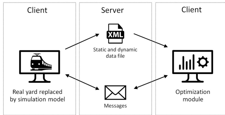
Figure 7: Closed-loop between optimisation and simulation
