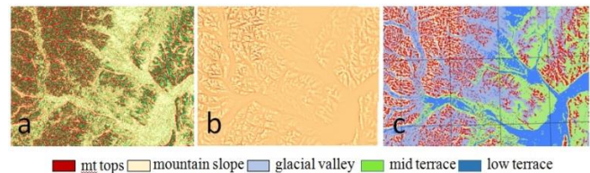
Fig. 2. a) TPI 250 m; b) TPI 500 m; c) landform classification Table 1. Landform Classification modified according to mesorelief characteristics:
