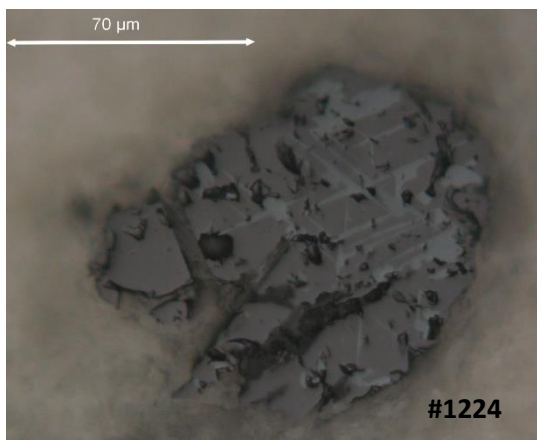
Supplementary Figure 2. Optical microphotographs in reflected light showing the diverse textures of the oxides within the serpentinite samples dehydrated at high-pressure.
