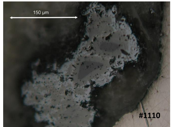
Supplementary Figure 2. Optical microphotographs in reflected light showing the diverse textures of the oxides within the serpentinite samples dehydrated at high-pressure.
