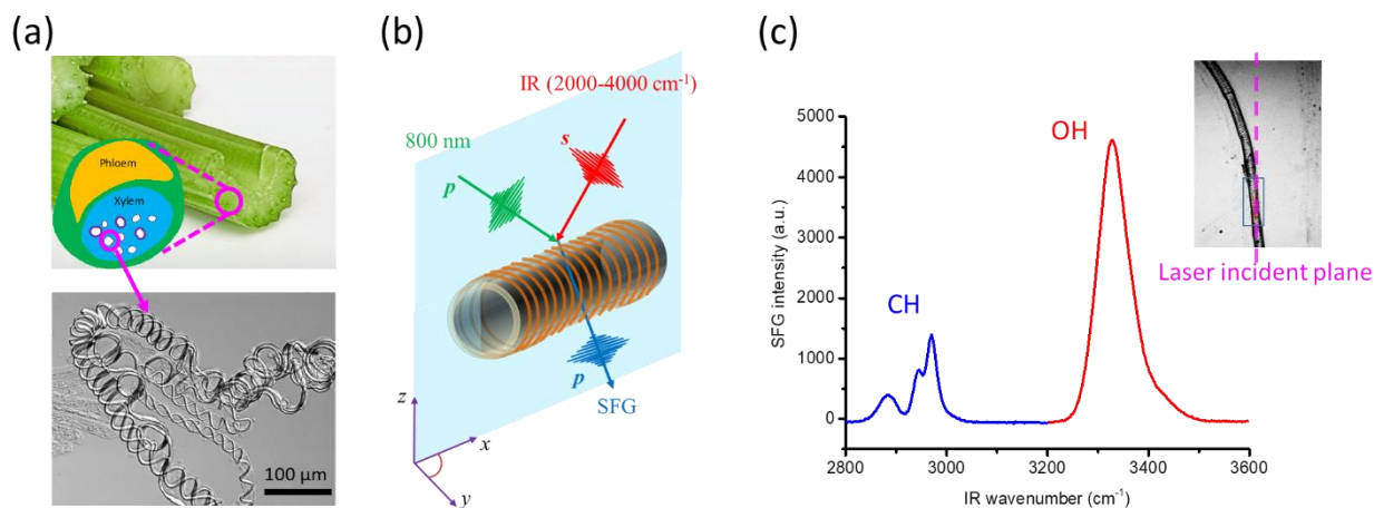
Figure 7. (a) Optical image of celery cross-section and the microscopic image of cellulose macrofibril coils isolated from the tracheary elements. (b) Experimental geometry of the transmission-SFG measurement. The coil axis is placed in the laser incidence plane and the SFG polarization combination is pps ; thus, the IR polarization is nearly parallel to individual cellulose microfibrils. (c) SFG spectrum of the cellulose macrofibril coil aligned along the laser incidence plane. The SFG spectrum of the coil aligned perpendicular to the laser incidence plane is shown in Figure S3.
