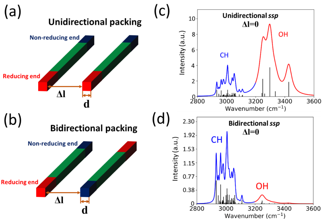
Figure 2. Schematic illustration of two cellulose crystallites in (a) unidirectional and (b) bidirectional packing and TD-DFT prediction of SFG spectral features for two crystals in intimate contact with (c) unidirectional and (d) bidirectional packing. The calculations were for crystalline domains consisting of cellobiose units with atomic positions in the cellulose I \beta coordinate. Note that the y-scale of the bidirectional packing case (d) is about 4 times smaller than the unidirectional case (c). 30, 39
