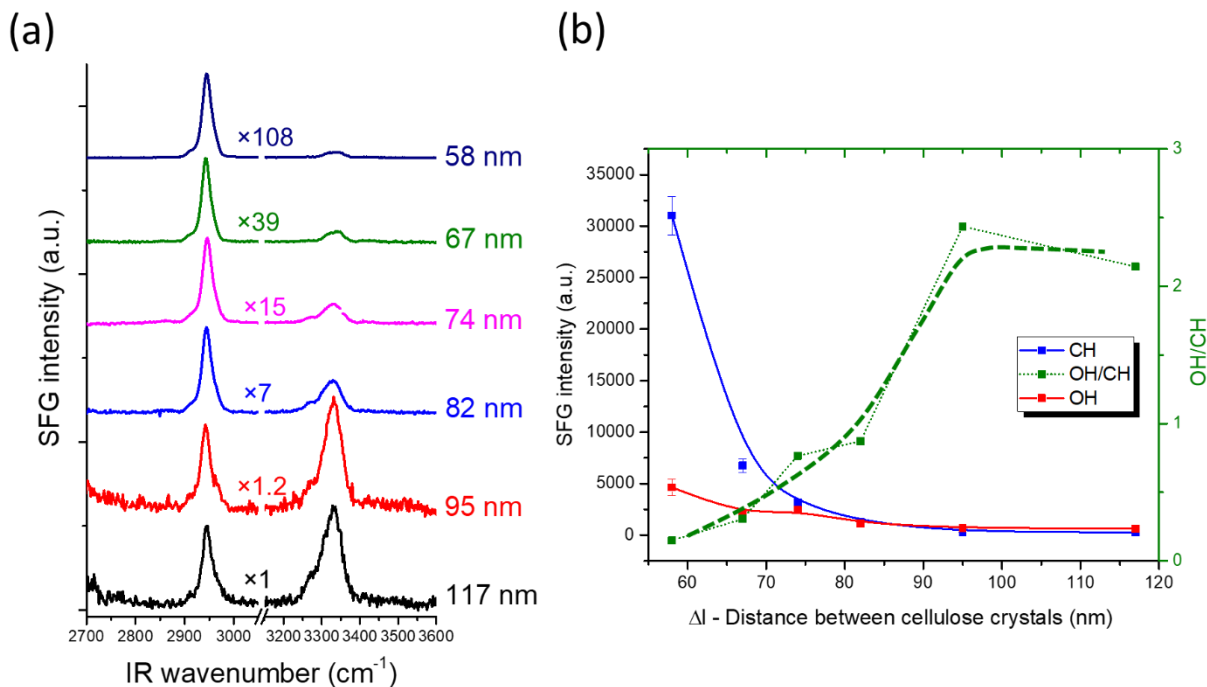
Figure 5. (a) SFG spectra of uniaxially-aligned CNCs dispersed in D 2 O in a rectangular capillary tube. The alignment direction is along the capillary tube. 58 The SFG spectra were collected in the reflection geometry with the ssp polarization; the number next to each spectrum is the relative intensity of the CH peak used for normalization of the spectrum for comparison. The inter-particle distance was calculated from the CNC concentration (see the Supporting Information). The directionality of CNCs in the suspension is random along the alignment axis, thus it is equivalent to the bidirectional packing in average over the coherence length scale. (b) Plots of CH and OH SFG areas (in the left y-scale) and the OH/CH ratio (in the right y-axis) Cellulose crystals extracted from tunicate were dispersed in D 2 O, where they form hexagonal arrays all aligned along the capillary tube.
