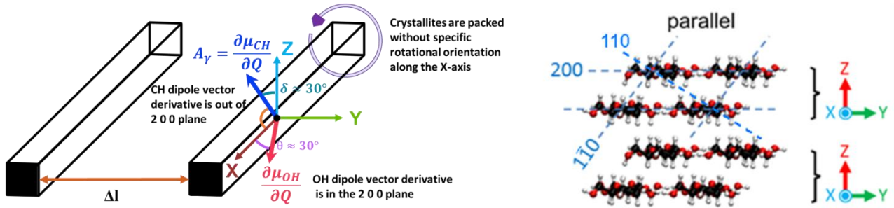
Figure 3. One-dimensional model for the theoretical calculation of the SFG intensity as a function of the interparticle separation distance ( \Delta l ). The image in the right shows eight chains of cellulose in the I \beta allomorph along the chain axis. When the (200) plane of cellulose I \beta is in the XY plane of the lab coordinate and the c-axis is aligned to the X-axis, the transition dipole moment of the CH stretch mode is assumed to be tilted by 60^\circ from the X-axis toward the Z-axis (away from the (200) plane; thus, \delta \approx 30^\circ ). The transition dipole moment of the OH stretch mode is tilted by 30^\circ from the chain axis toward the Y-axis (within the (200) plane). These angles are chosen for the simulation based on the TD-DFT calculations and the polarization IR measurements. 30, 39-40 The right image is copied from Ref. 39 with permission conveyed from Copyright Clearance Center Inc.
