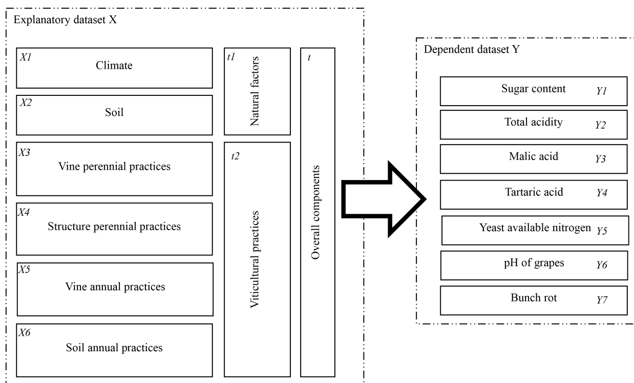
FIGURE 1. Graphical representation of the block and group datasets showing the relationships between the blocks of variables with t the common component for all individuals.
