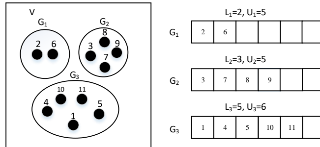
Fig. 1. An illustrative example for solution representation with N = 11 , m = 3 , and U_{max} = 6 . We use a 3 \times 6 matrix A (right figure) to indicate a solution (left figure).
