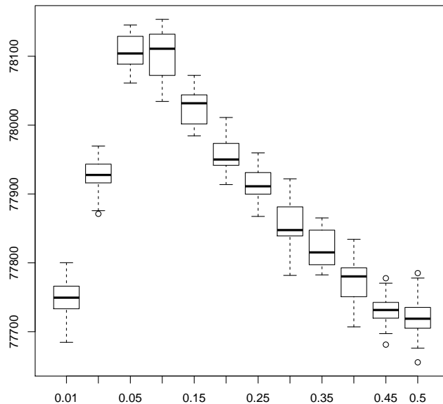
Fig. 6. Sensitivity analysis of parameter \mu based on the 20 EGS instances with N = 2000 and m = 200 , where the X-axis indicates the parameter values and the Y-axis shows the average objective values ( f_{avg} ) obtained over 20 independent runs.
