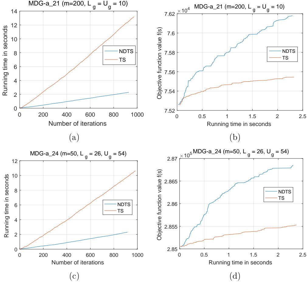
Fig. 4. Comparison between NDTs and TS in terms of the objective function value f(s) and the running time.
