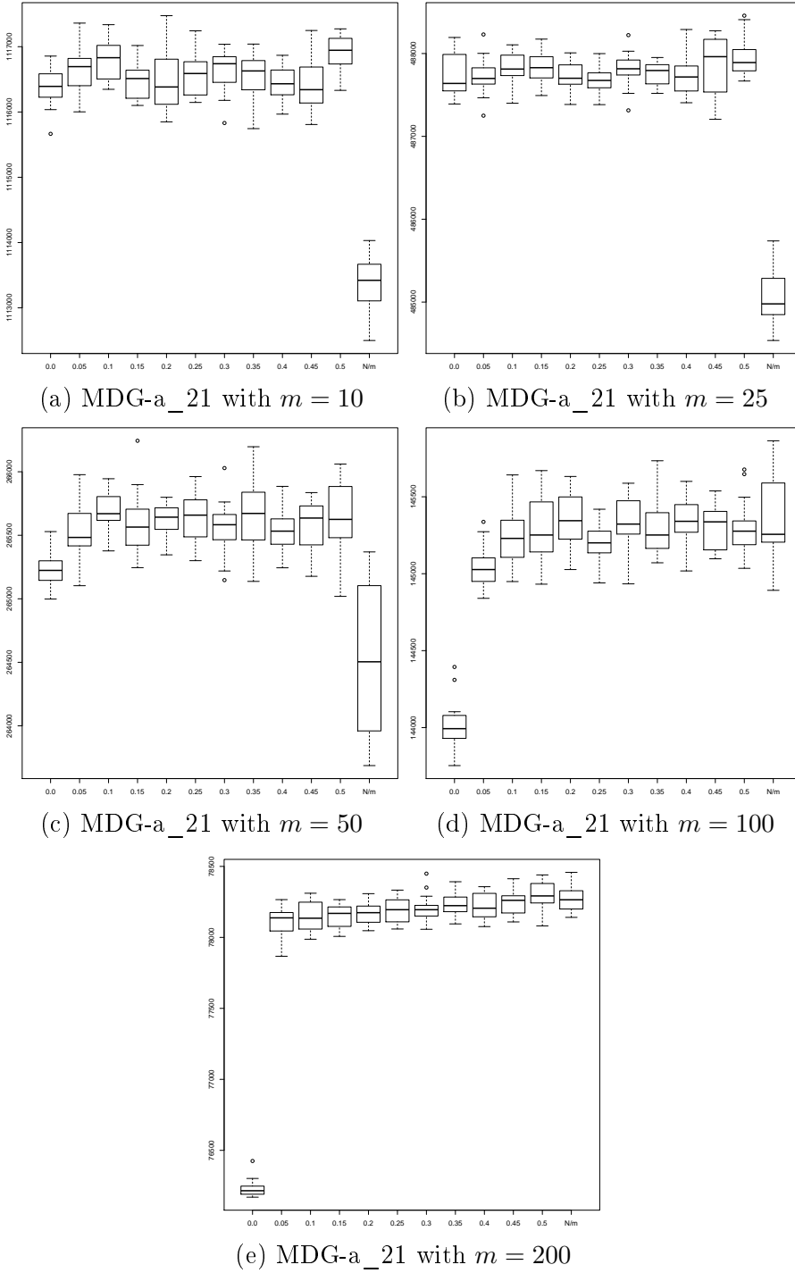
Fig. 5. Sensitivity analysis for the parameter Q used to control the probability that the NDTS procedure is applied. The X-axis indicates the settings of Q and the Y-axis indicates the objective value.
