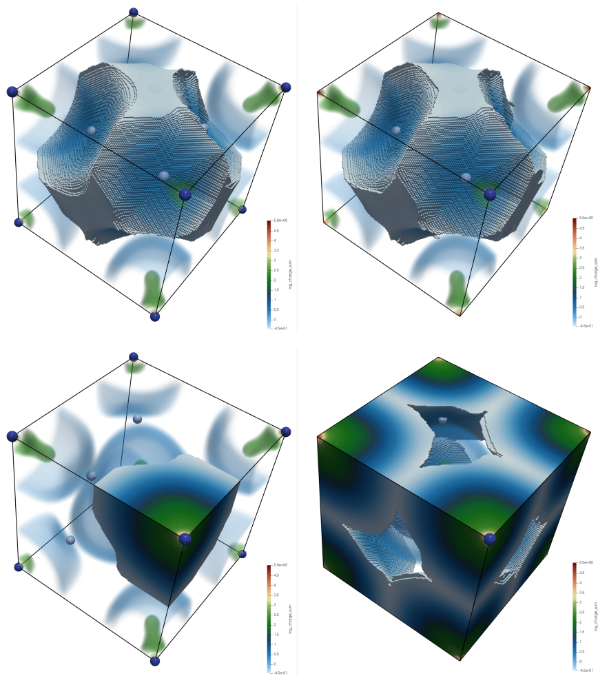
Fig. 8 Results of the Morse-Smale complex computation for a methane crystal modeled via a fixed unit cell that contains two methane molecules with a non-periodic (left) and a periodic (right) boundary. (First row) One methane molecule is located in the middle of the domain and hence it is correctly identified as an ascending manifold of a maximum in the Morse-Smale complex with or without periodic boundaries. (Second row) However, for the molecule located at the corner of the cell, the ascending manifold with periodic boundary correctly identifies the region corresponding to the second molecule. The ascending manifold without periodic boundary fails to correctly segment the volume into two methane molecules.
