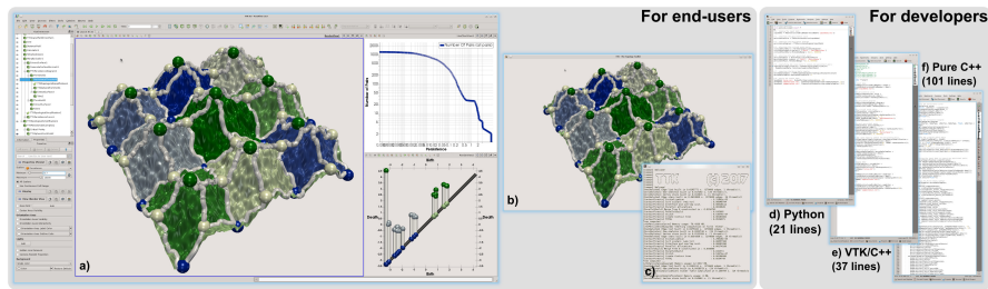
Fig. 1 TTK is a software platform for topological data analysis and scientific visualization. It is both accessible to end-users—via ParaView plugins (a), VTK-based generic GUIs (b), and command-line programs (c)—and to developers—via Python (d), VTK/C++ (e) or dependence-free C++ (f) bindings. TTK provides an efficient and unified approach to topological data representation and simplification, which enables in this example a discrete Morse-Smale complex (a) to comply to the level of simplification dictated by a piecewise linear persistence diagram (bottom-right linked view, a). Code snippets are provided (d-f) to reproduce this pipeline.
