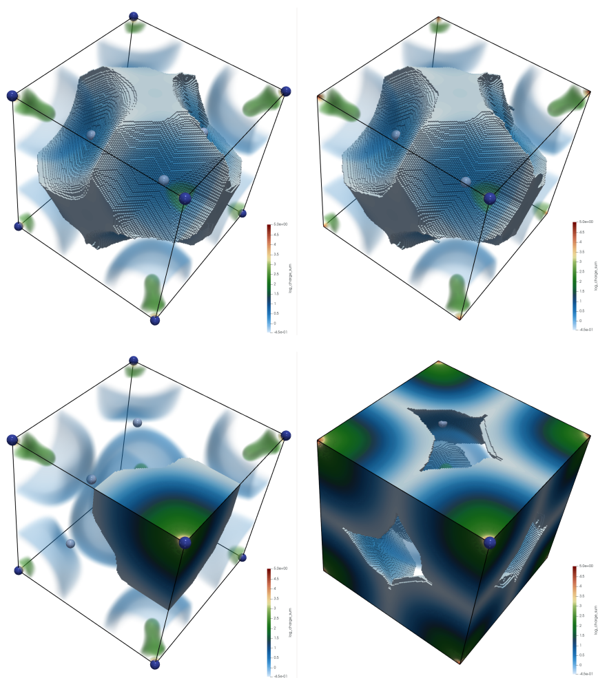
Fig. 8 Results of the Morse-Smale complex computation for a methane crystal modeled via a fixed unit cell that contains two methane molecules with a non-periodic (left) and a periodic (right) boundary. (First row) One methane molecule is located in the middle of the domain and hence it is correctly identified as an ascending manifold of a maximum in the Morse-Smale complex with or without periodic boundaries. (Second row) However, for the molecule located at the corner of the cell, the ascending manifold with periodic boundary correctly identifies the region corresponding to the second molecule. The ascending manifold without periodic boundary fails to correctly segment the volume into two methane molecules.
