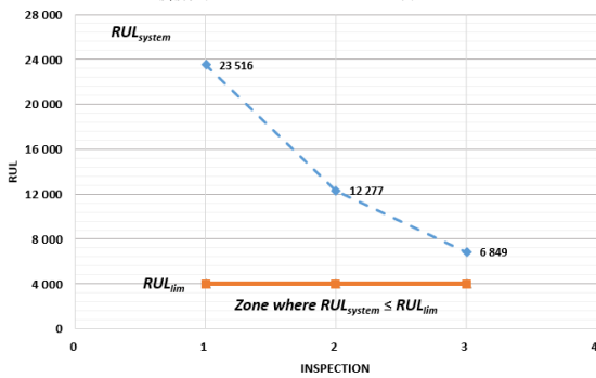
Figure 8. Variation of RUL_{system} , case N_{in}=3
