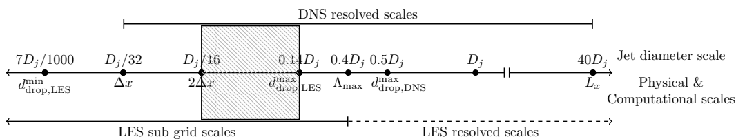
Figure 6: Schematic of range of length scales of motion resolved by DNS and LES at x/D_j = 20 with shared length scales shown in hatched region.
