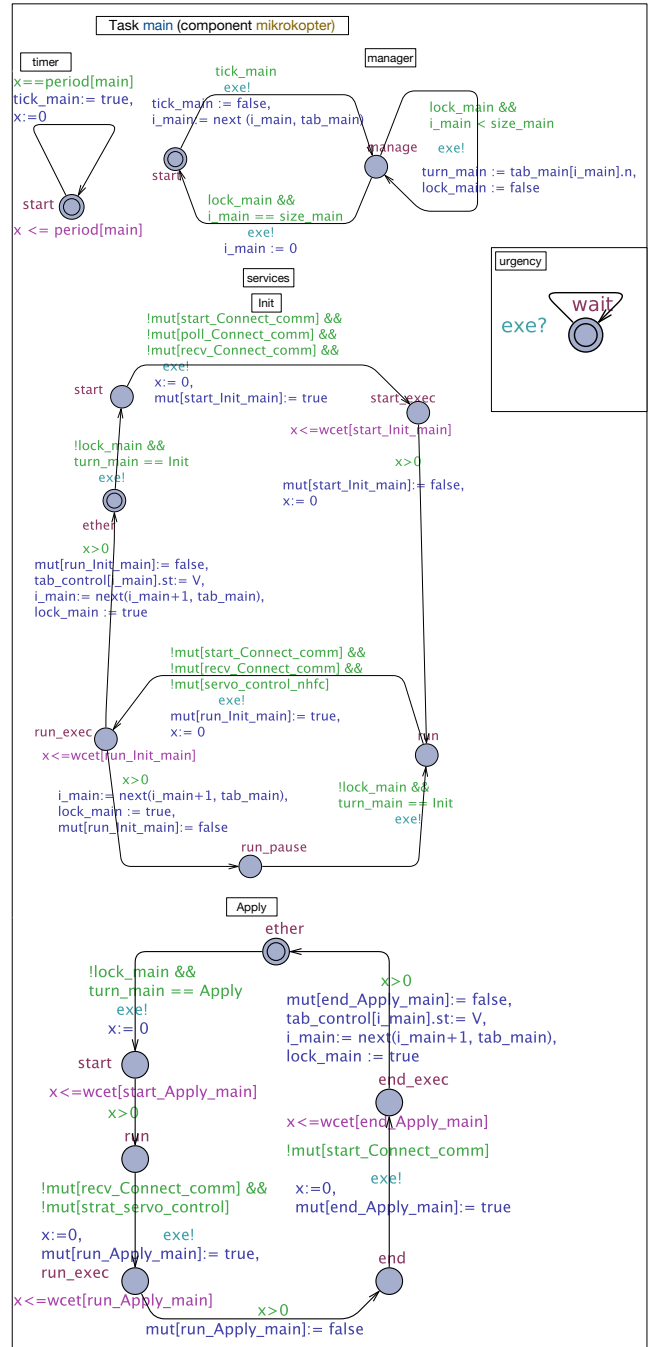
Fig. 3: Simplified UPPAAL model of task main in component MIKROKOPTER. Process Urgency does not belong to any component and is added to enforce urgencies, i.e. prevent unnecessary lazy waits (the receiver (?) edge is always ready).
