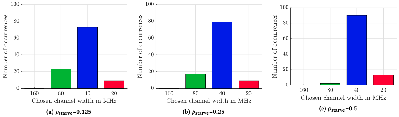
Figure 6: Histograms of the channel width chosen by our proposed solution for the 105 considered physical conflict graphs.
