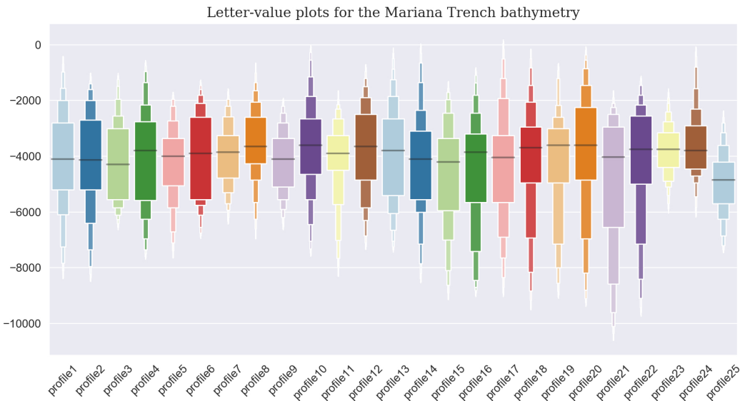
Fig.11 Letter-value plot for data distribution, Mariana Trench bathymetric profiles. Plotting: Seaborn library, Python. (Source: author).
