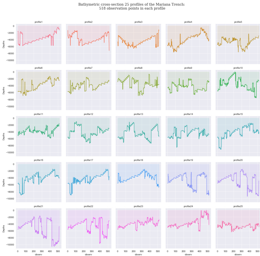
Fig. 9 Area chart and facet grid of the 25 cross-section bathymetric profiles of the Mariana Trench. Plotting visualization: Seaborn library, Python. (Source: author).
