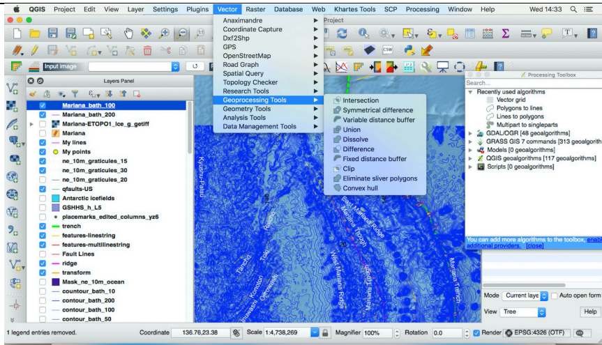
Fig. 6 Geoprocessing of bathymetric layer in Quantum GIS (Source: author).
