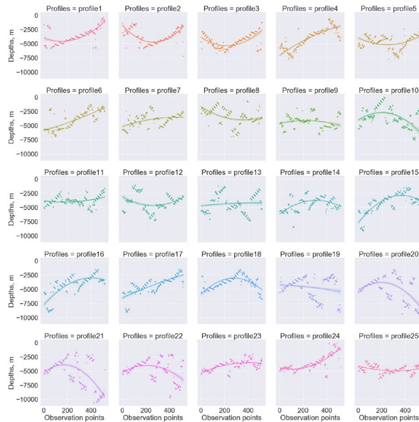
Fig.10 Regression analysis: facet grid of the 25 cross-section bathymetric profiles of the Mariana Trench. Plotting visualization: Seaborn library, Python. (Source: author).
