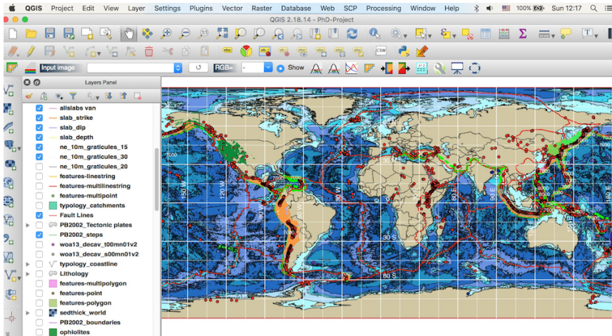
Fig. 5 QGIS project showing map layers visualization (Source: author).
