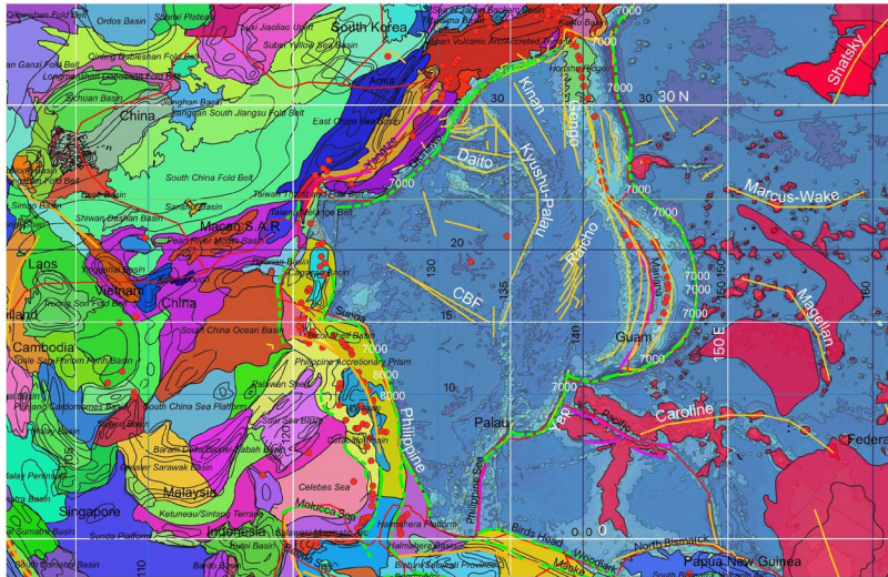
Fig. 3 Geological provinces and ophiolites (Source: author).
