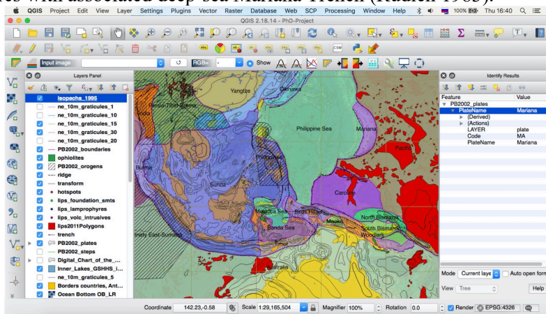
Fig. 2 Tectonic plates boundaries, QGIS project (Source: author).
