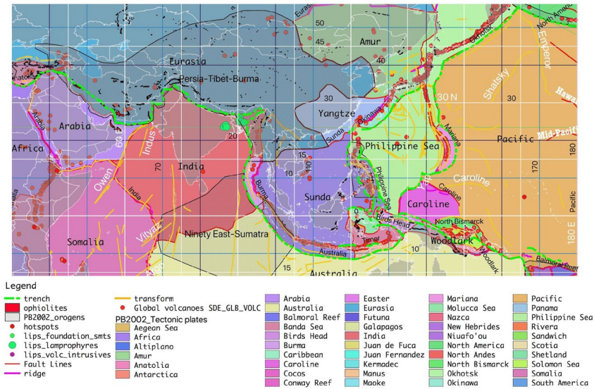
Fig. 4 Tectonic provinces and minor tectonic plates (Source: author).
