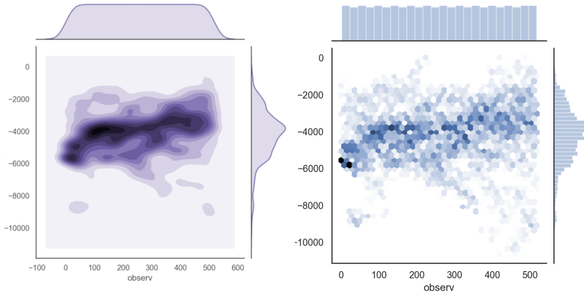
Fig.12 Hexagonal and KDE plots. Plotting: Python. (Source: author).
