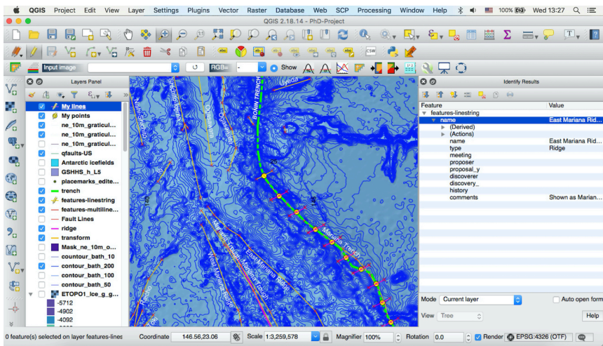
Fig. 7 Digitizing central points of 25 profiles in Quantum GIS (Source: author).
