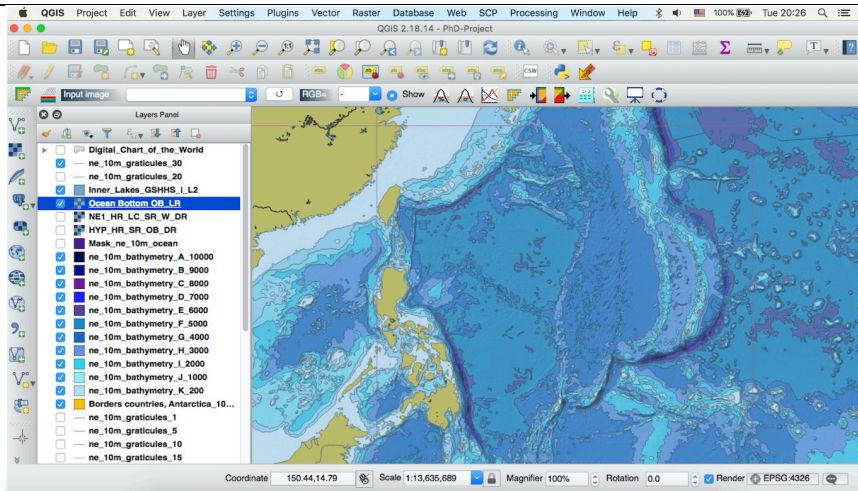
Fig. 1 Study area: crescent arc of the Mariana Trench (Source: author).
