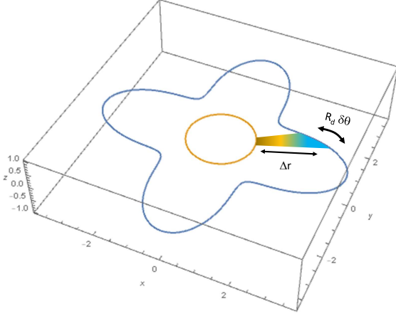
FIG. 4: (Color online) Normalized stretching function \epsilon plotted for mode \{n=2, m=1\} in high-stress limit (with z_{n,m}/R_d = 1 ). The stretched surface area R_d \delta\theta \Delta r is indicated on the graph (central circle represents the drum).
