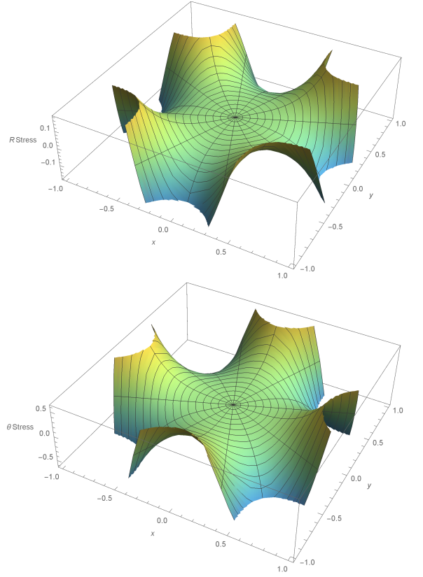
FIG. 5: (Color online) Stress components \sigma_r^{angl.} (top) and \sigma_\theta^{angl.} (bottom) computed for mode \{n=2, m=1\} in the high-stress limit. The graph has been normalized to E_r = 1 , R_d = 1 , and z_{n,m}/R_d = 1 (using \nu_r = +0.3 ).
